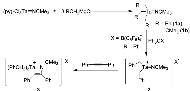
Scheme 1. Synthesis of Neutral and Cationic Alkyl Tantalum Imido Complexes
