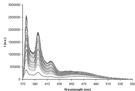
Figure 3. Variation in the emission spectra of 1 upon successive additions of METH variations: [\textbf{1}] = 10 \mu\text{M} , [\text{METH}] = 1\text{--}100 \mu\text{M} , \lambda_{\text{exc}} = 342 \text{ nm} .
