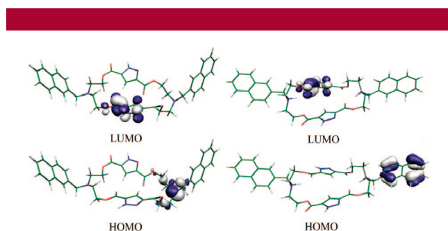
Figure 2. Electronic density contours ( 0.05 \text{ e bohr}^{-3} ) calculated for the frontier molecular orbitals (HOMO and LUMO) of 2 (left) and 2HH (right) in their singlet ground states.
