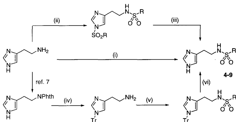
Scheme 1. (i) \text{RSO}_2\text{Cl} (1 equiv.), \text{Et}_3\text{N} , DMF; (ii) \text{RSO}_2\text{Cl} (2 equiv.), \text{Et}_3\text{N} , \text{CH}_2\text{Cl}_2 ; (iii) \text{Na}_2\text{CO}_3 , \text{H}_2\text{O} , EtOH; (iv) (a) \text{Ph}_3\text{CCl} , \text{Et}_3\text{N} , \text{CH}_2\text{Cl}_2 , (b) \text{NH}_2\text{NH}_2 \cdot \text{H}_2\text{O} , EtOH, reflux; (v) \text{RSO}_2\text{Cl} , \text{Et}_3\text{N} , \text{CH}_2\text{Cl}_2 ; (vi) \text{CF}_3\text{CO}_2\text{H} .
