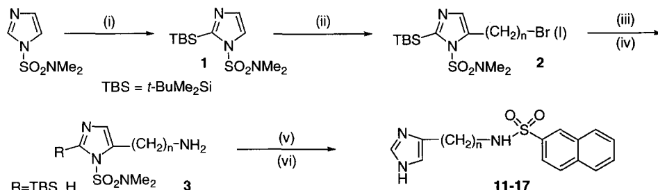
Scheme 2. (i) (a) n\text{-BuLi} , THF, (b) \text{TBSCl} ; (ii) (a) n\text{-BuLi} , THF, (b) \text{Br}(\text{CH}_2)_n\text{Br} ( \text{Cl}(\text{CH}_2)_n\text{I} ); (iii) \text{KNPhth} , DMF, 100^\circ\text{C} ; (iv) \text{NH}_2\text{NH}_2 \cdot \text{H}_2\text{O} , EtOH, reflux; (v) 2-Naphth \text{SO}_2\text{Cl} , \text{Et}_3\text{N} , \text{CH}_2\text{Cl}_2 ; (vi) 2M \text{HCl} , EtOH, reflux.
