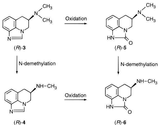
Scheme 1. Structures and Metabolic Pathway for Methylamine Analogues
