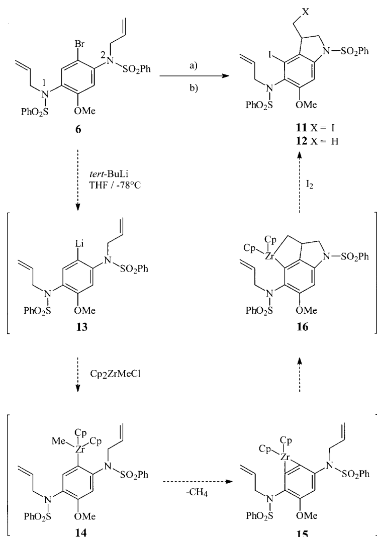
Scheme 3. Mechanism of the zirconocene-induced cyclization. Reaction conditions: a) t BuLi, \text{Cp}_2\text{ZrMeCl} , THF, 19 h, -78 \rightarrow 20^\circ\text{C} ; b) 2 equiv \text{I}_2 , \text{CH}_2\text{Cl}_2 , 60% \rightarrow 11 , or \text{I}_2 , HCl, \text{CH}_2\text{Cl}_2 , \text{H}_2\text{O} \rightarrow 12 .
