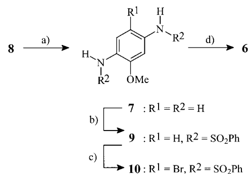
Scheme 2. Synthesis of compound 6 . Reaction conditions: a) \text{PtO}_2/\text{H}_2 , dioxane, 18 h, 3 bar, quant.; b) \text{PhSO}_2\text{Cl} , pyridine, 3 h, 80 °C, 77 %; c) NBS, THF, –78 → 20 °C, 95 %; d) NaH, THF, 1 h, 20 °C; allyl bromide, n\text{Bu}_4\text{NI} , 5 h, 50 °C, 95 %.
