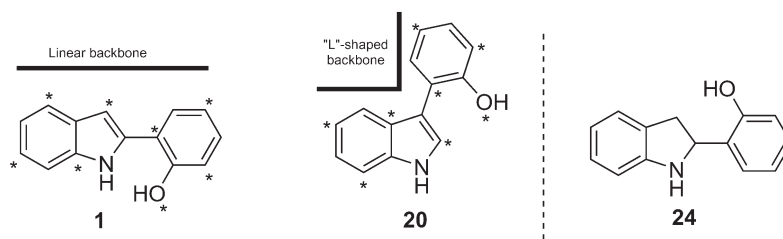
Fig. 5 The possible locations of a delocalised phenol radical, identified by an asterisk (*), on 1 and 20 (left); and an analogue of 1 with reduced conjugation, 24 (right).
