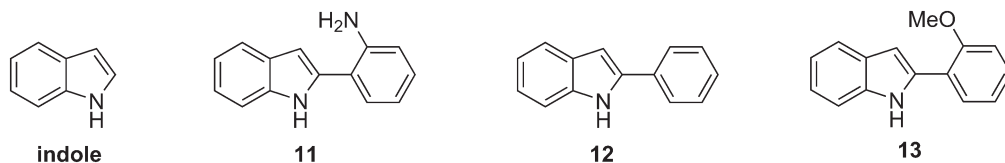
Fig. 3 Analogues used to probe the importance of the phenol group.
