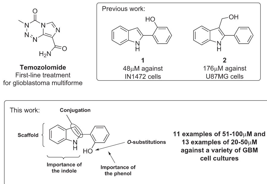
Fig. 1 Structure of the first-line treatment temozolomide for malignant brain tumours of the type glioblastoma multiforme (GBM), and two 2-aryl indoles from our previous work on anti-glioblastoma lead compounds. 3 The work described herein is depicted by the box entitled 'This work' showing the features of 1 that were studied and some selected \text{EC}_{50} values.
