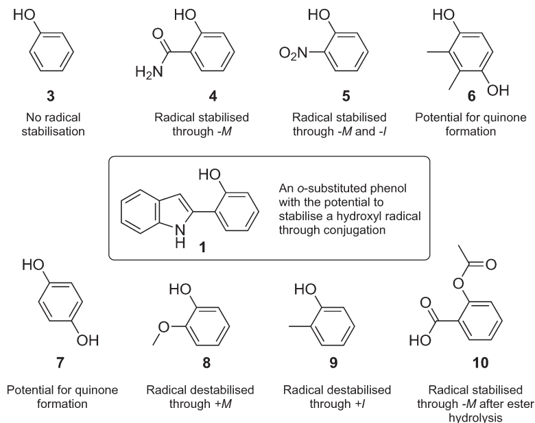
Fig. 2 The series of phenols tested in order to establish the importance of the indole group. 10 is assumed to hydrolyse to the phenol in the cell. M and I represent mesomeric and inductive effects, respectively.
