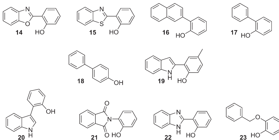
Fig. 4 The analogues tested with different scaffolds to that of 1. EC 50 s can be seen in Table 3.
