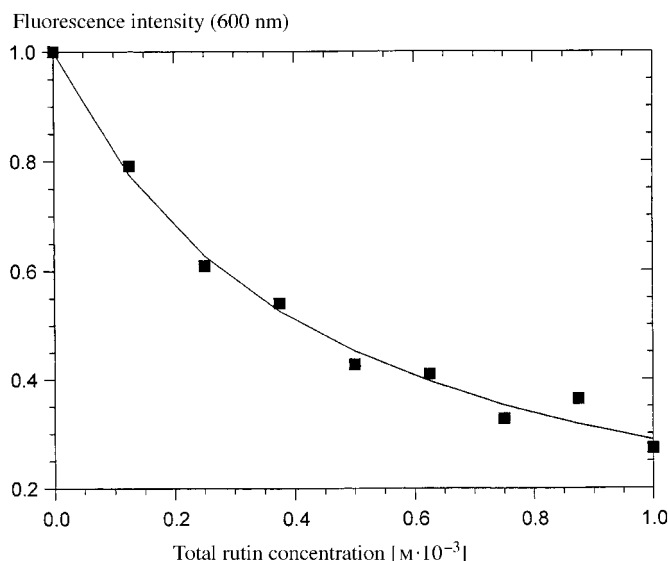
Fig. 3. Plot of the fluorescence intensity of malvin at 600 nm (excitation at 540 nm) as a function of the total rutin concentration (pH 0.9, 25°). The solid line is the result of the curve-fitting procedure according to Eqns. 3 and 4.
