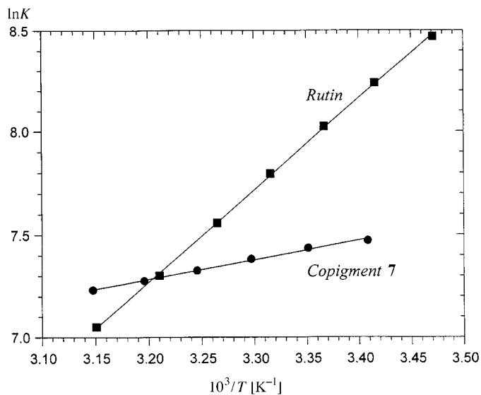
Fig. 2. Van't Hoff plots for copigmentation of malvin ( 5 \cdot 10^{-5} \text{M} ) by rutin ( 10^{-3} \text{M} ) and rutin derivative 7 ( 10^{-2} \text{M} ) at pH 3.5 (0.2M acetate buffer)
