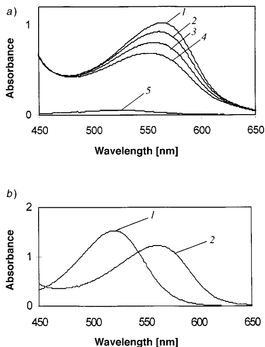
Fig. 1. Copigmentation of malvin ( 5 \cdot 10^{-5} \text{M} ) by rutin derivative 6 ( 10^{-2} \text{M} ). a) At pH 3.5 (0.2M acetate buffer), VIS spectra of malvin/6 at 15.5 (1), 25.0 (2), 35.0 (3) and 44.2° (4); VIS spectrum of malvin alone at 25.3° (5). b) At pH 0.9 and 25°, VIS spectrum of malvin alone (2) and of malvin/6 (1)
