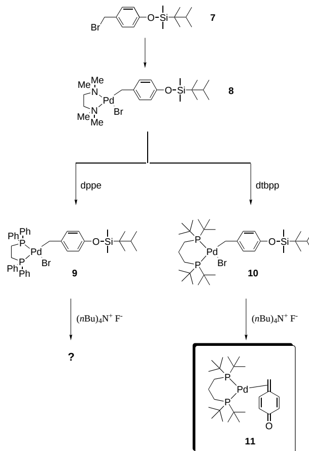
Scheme 9. Formation of the novel Pd^0 complex of s-QM ( 11 ).
