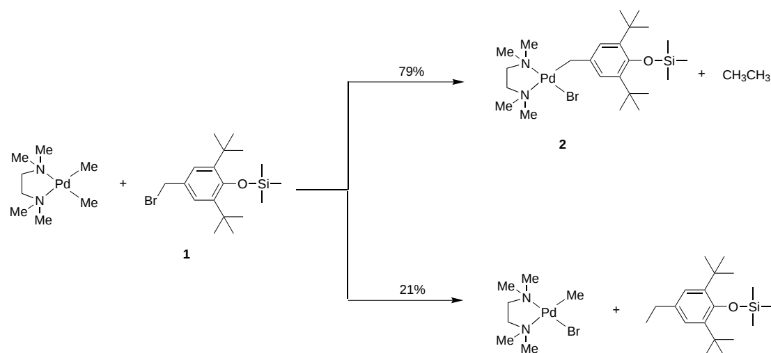
Scheme 3. Reaction of 1 with [(tmeda)PdMe 2 ].
