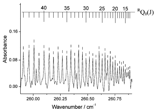
Figure 1. The J -assignment of the assumed ^RQ_0 -branch in the \nu_9^1 band of \text{H}_3\text{N}-\text{HCN} .
