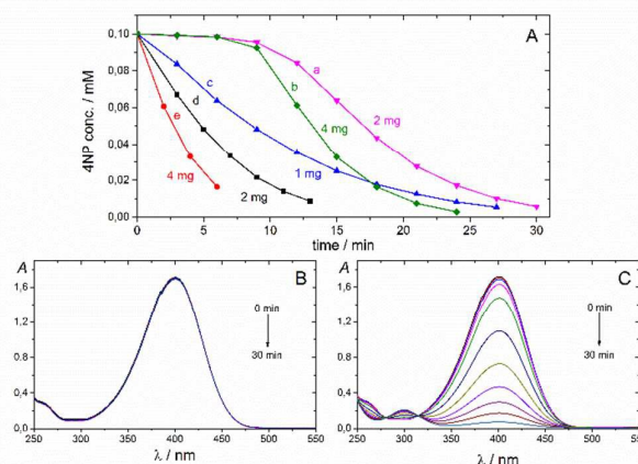
Fig. 4. Concentration of 4NP versus time for the 4NP reduction by NaBH 4 at the presence of Cu-NP/C microspheres (A) (amount of catalyst used is indicated; initial 4NP and NaBH 4 concentrations are 0.1 and 10 mM; catalyst was added to mixed solutions of 4NP and NaBH 4 (a and b); 4NP solution stirred with the catalyst for 10 min before adding NaBH 4 solution (c, d and e), temperature = 20 °C). Time dependent evolution of UV/Vis spectra of 4NP anion at the absence (B) and at the presence (C) of Cu-NP/C catalyst showing the reduction of 4NP by NaBH 4 .
