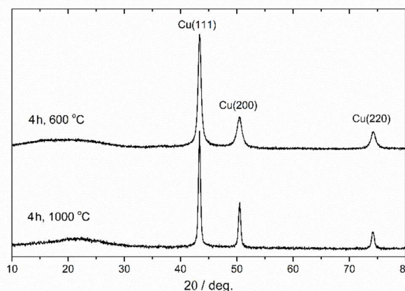
Fig. 1. Powder X-ray diffractogram of selected Cu-NP/C microspheres (carbonisation time and temperature is indicated).
