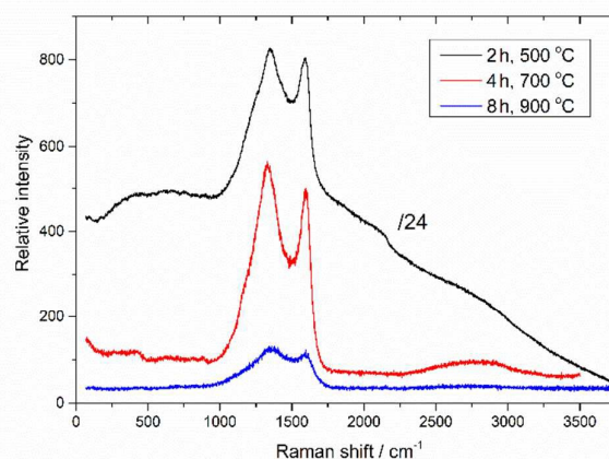
Fig. 2. Raman spectra of selected Cu-NP/C microspheres (carbonisation time and temperature is indicated, see also Figure S3, ESI).
