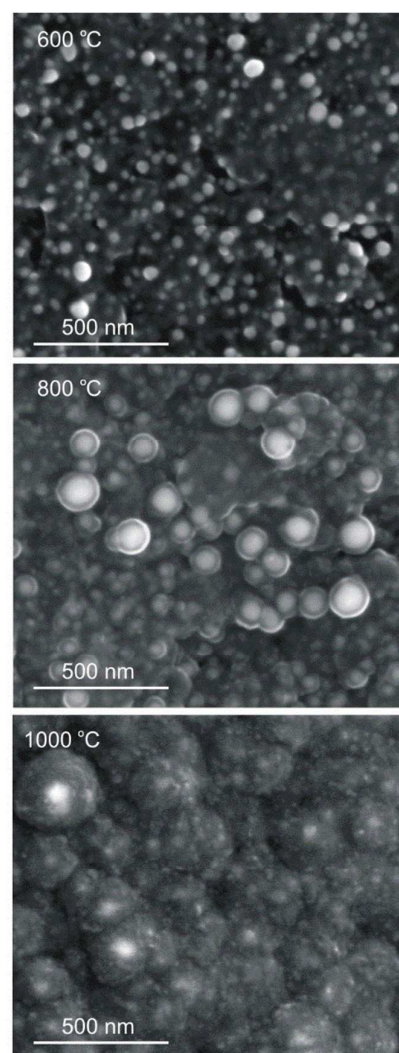
Fig. 3. SEM image of the Cu-NP/C microsphere surface obtained by carbonisation of the copper loaded ion exchange resin at 600, 800, and 1000 °C for 8h (see also Figure S5-7, ESI).
