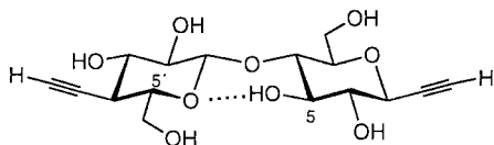
Fig. 1. Structure of the deprotected monomer 1 (adapted from [4]). The dotted line indicates the C(5′)–O···HO–C(5) intramolecular H-bond.
