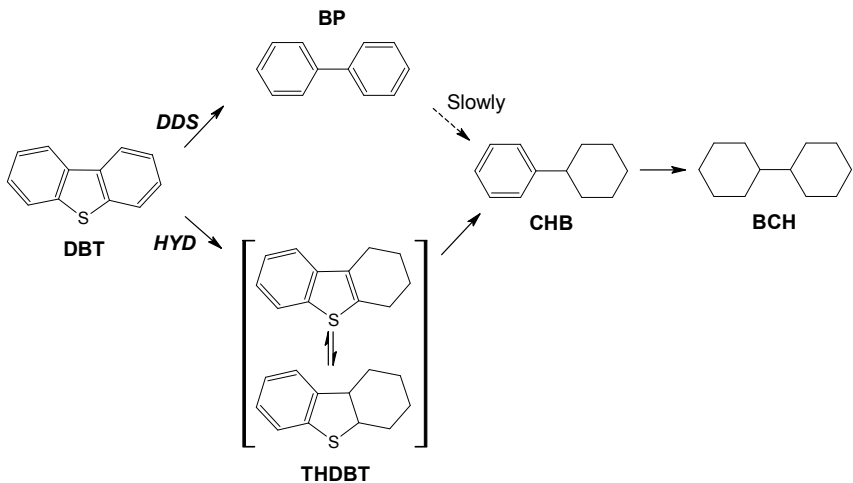
Scheme 1. Reaction network of the HDS of DBT.
