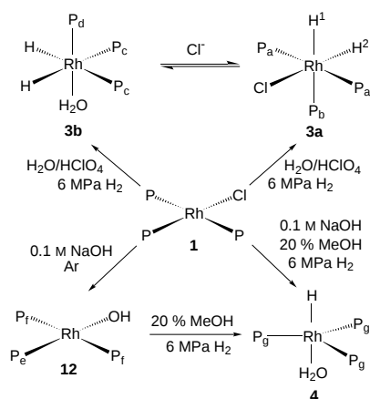
Scheme 1. Hydrolysis and hydrogenation equilibria in the aqueous solution of [RhCl(tppms) 3 ] ( 1 ) under argon or hydrogen. P = TPPMS ( 8 ).
