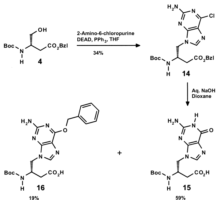
Scheme 3. Synthesis of the Guaninyl- \beta -amino Acid 15 from the \beta -Homoserine Derivative 4 with the Mitsunobu Reaction as the Key Step
