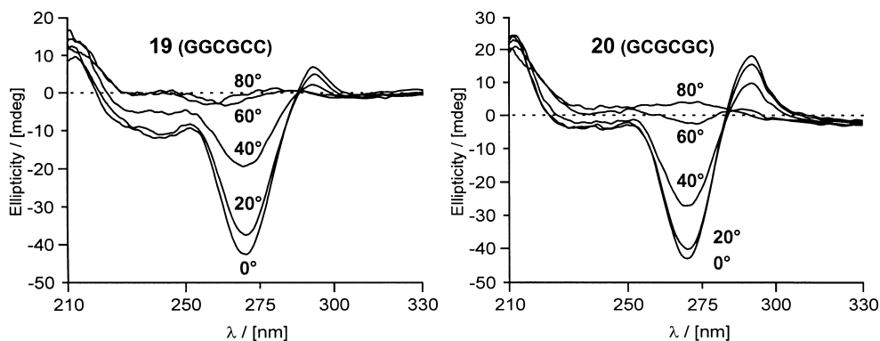
Fig. 2. CD Spectra of oligomers 19 (left, 10 \mu M in H 2 O) and 20 (right, 12 \mu M in H 2 O)
