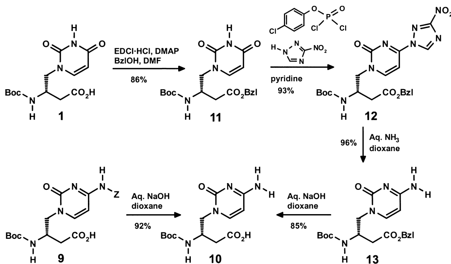
Scheme 2. Conversion of the Uracilyl- \beta -amino Acid 1 into the Unprotected Cytosinyl- \beta -amino Acid 10 to Establish the Connectivity of the Protected Cytosinyl- \beta -amino Acid 9
