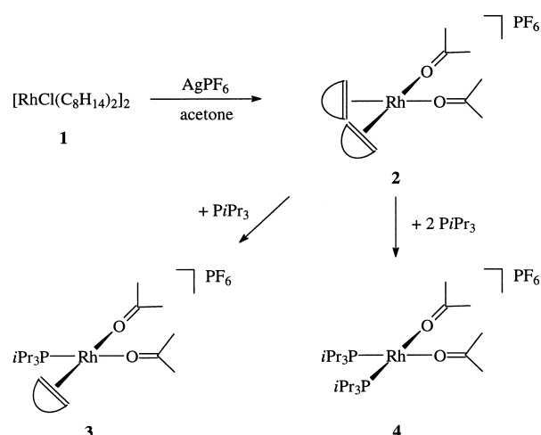
Scheme 1. Preparation of the cationic bis(acetone)rhodium(I) complexes 2 – 4 from the bis(cyclooctene) complex 1 .
