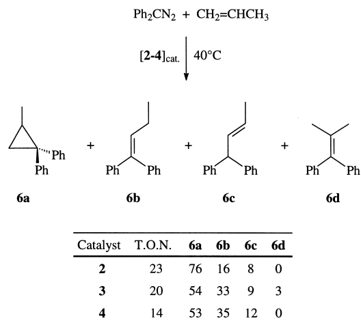
Scheme 3. Results of the catalytic reaction of propene and Ph 2 CN 2 with compounds 2–4 as catalyst (T.O.N. = turnover number = [(mmol product)/(mmol catalyst)]); ratio of 6a , 6b , 6c , and 6d in %).
