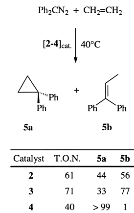
Scheme 2. Results of the catalytic reaction of ethene and Ph 2 CN 2 with compounds 2–4 as catalyst (T.O.N. = turnover number = [(mmol product)/(mmol catalyst)]); ratio of 5a and 5b in %).
