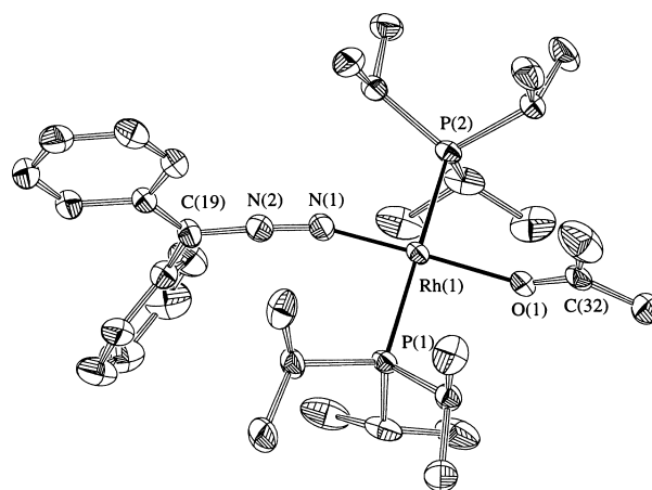
Figure 2. Molecular structure of 8 (anionic ligand omitted for clarity). Principal bond lengths [Å] and angles [ ^\circ ] with estimated standard deviations in parentheses: Rh(1)–P(1) 2.3546(8), Rh(1)–P(2) 2.3693(8), Rh(1)–O(1) 2.039(2), Rh(1)–N(1) 1.869(3), N(1)–N(2) 1.157(4), N(2)–C(19) 1.312(4), O(1)–C(32) 1.237(4); P(1)–Rh(1)–P(2) 170.88(3), P(1)–Rh(1)–O(1) 90.36(6), P(1)–Rh(1)–N(1) 91.71(8), P(2)–Rh(1)–O(1) 89.47(6), P(2)–Rh(1)–N(1) 87.29(8), O(1)–Rh(1)–N(1) 172.21(10), Rh(1)–O(1)–C(32) 140.1(2), Rh(1)–N(1)–N(2) 161.0(2), N(1)–N(2)–C(19) 171.6(3).
