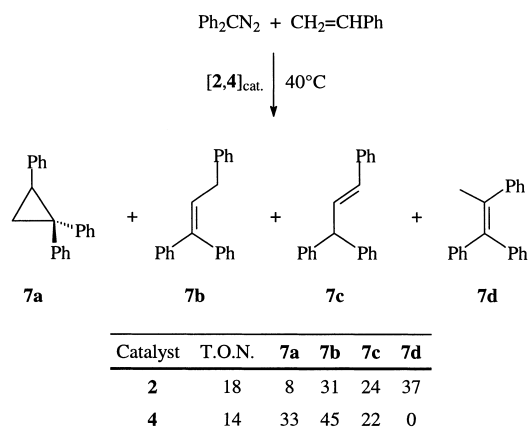
Scheme 4. Results of the catalytic reaction of styrene and Ph 2 CN 2 with compounds 2–4 as catalyst (T.O.N. = turnover number = [(mmol product)/(mmol catalyst)]); ratio of 7a , 7b , 7c , and 7d in %).
