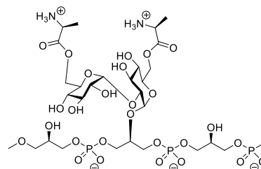
Figure 1. The structure of E. faecalis D-alanine kojibiose functionalized LTA.
