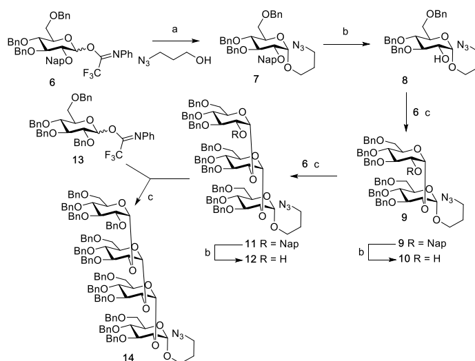
Scheme 2. The assembly of kojiligosaccharides. a) TMSI, Ph_3P=O , DCM, 36 h, 75%, \alpha:\beta = 10:1 . b) DDQ, DCM: H_2O = 10:1 (v/v), 8 : 75%; 10 : 49%; 12 : 47%. c) DMF, TfOH, DCM, 9 : 95%, \alpha:\beta = 15:1 ; 11 : 67%, \alpha:\beta = 10:1 ; 14 : 67%, \alpha:\beta = 2:1 .
