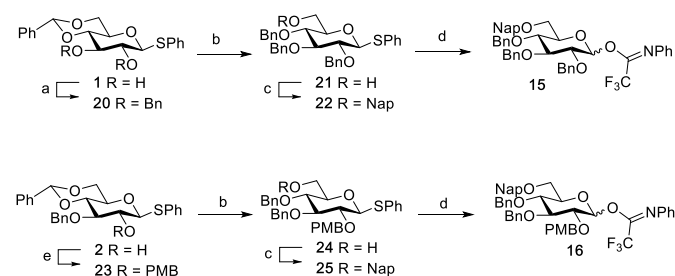
Scheme 4. Synthesis of donor 15 and 16 . a) BnBr, NaH, DMF, 20 : 96%. b) \text{BH}_3\cdot\text{THF} , \text{Cu}(\text{OTf})_2 , 21 : 80%; 24 : 76%. c) NapBr, NaH, DMF, 22 : 91%; 25 : 93%. d) 1) NIS, acetone: \text{H}_2\text{O} = 10:1 (v:v); 2) 2,2,2-trifluoro- N -phenylacetimidoyl chloride, \text{Cs}_2\text{CO}_3 , acetone, yield 15 : 86%; 16 : 84%. e) PMBCl, NaH, DMF, 94%.
