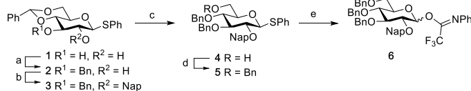
Scheme 1. Synthesis of donor 6 . a) i) Bu_2SnO , Toluene, 120 °C; ii) CsF , BnBr , 76%. b) NapBr , NaH , DMF, 91%. c) BF_3 \cdot Et_2O , TES, DCM. d) BnBr , NaH , DMF, 88%. e) i) NIS, Acetone/ H_2O (10:1, v/v); ii) 2,2,2-trifluoro- N -phenylacetimidoyl chloride, Cs_2CO_3 , acetone, 81% (over two steps).
