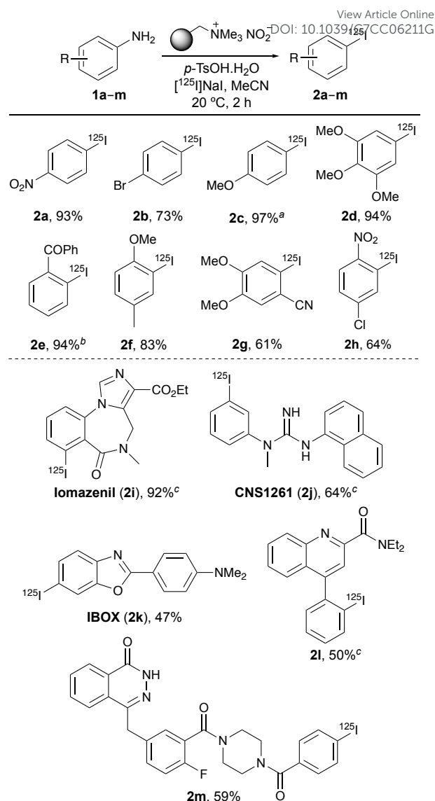
Scheme 1 Scope of one-pot diazotisation-radioiodination. a Reaction was performed at 40 °C. b Reaction required 4 h. c Reaction was performed at 60 °C
