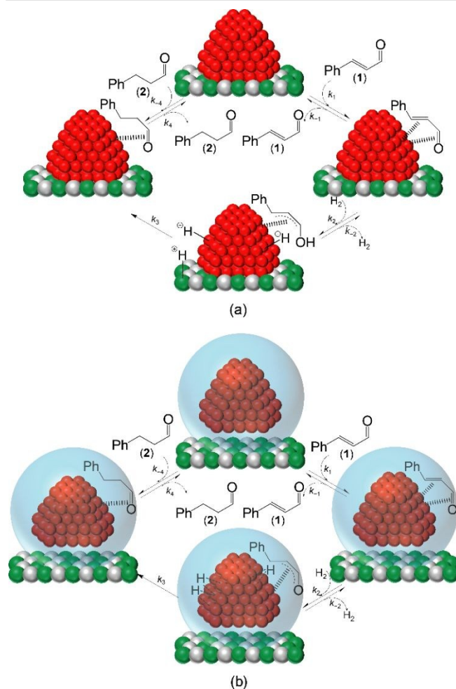
Scheme 4. Proposed mechanism for the hydrogenation of 1 catalyzed by (a) Au/γ-Al 2 O 3 , and (b) Au/M1 and Au/M2. Adapted from reference 18.
