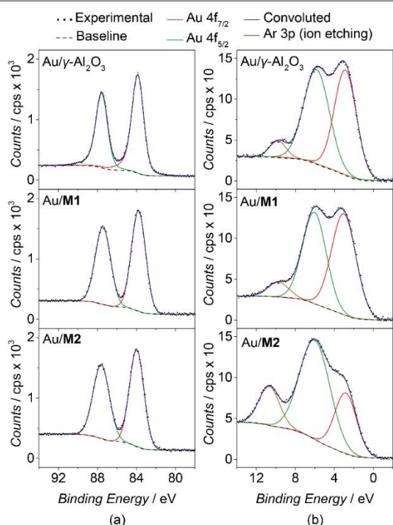
Figure 1. XPS measurements at (a) Au 4f and (b) Au valence band regions on the Au/ \gamma -Al 2 O 3 , Au/ M1 , and Au/ M2 catalysts.
