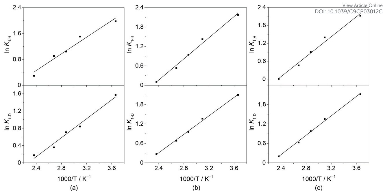
Figure 5. Van't Hoff plots of the hydrogenation and deuteration of 1 catalyzed by (a) Au/γ-Al 2 O 3 , (b) Au/M1, and (c) Au/M2.
