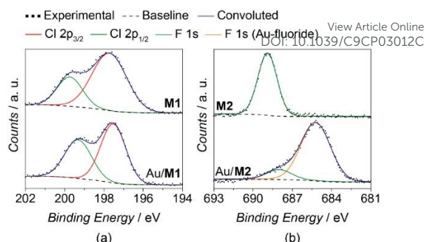
Figure 2. XPS spectra at (a) the Cl region of the M1 support and Au/ M1 catalyst and (b) the F region of the M2 support and Au/ M2 catalyst.
