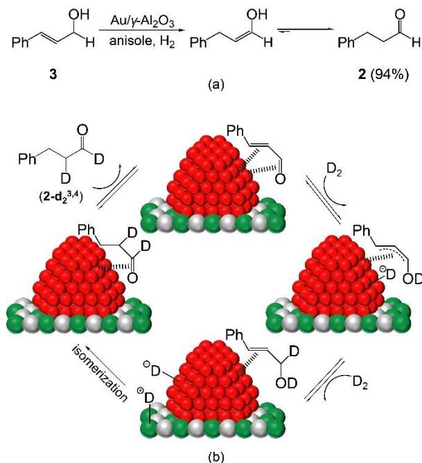
Scheme 2. Isomerization of (a) 3 and (b) 3-d 2 catalyzed by Au/γ-Al 2 O 3 . Reaction conditions: Au (0.5 μmol), substrate/Au = 1000, anisole (10 mL), 2.5 MPa of H 2 or D 2 , 273 K, and 250 rpm. Adapted from reference 18.
