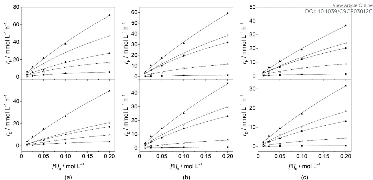
Figure 3. Hydrogenation and deuteration rate dependence on 1 concentrations catalyzed by (a) Au/ \gamma -Al 2 O 3 , (b) Au/M1, and (c) Au/M2 at temperatures of 273 K (■), 323 K (□), 348 K (●), 373 K (○), and 423 K (▲).
