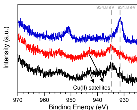
Figure 1. Comparison between Cu 2p HR-XPS spectra for Cu@Charcoal untreated (black) and treated by Method 1 (red) and Method 2 (blue).
