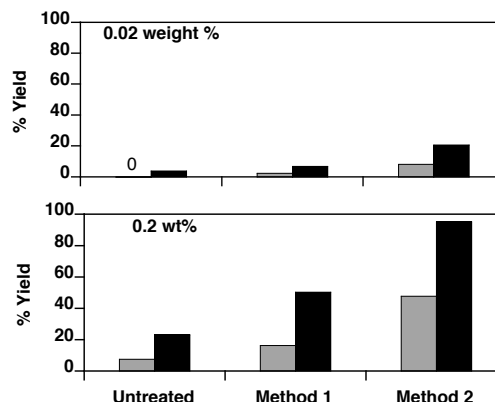
Figure 2: Yields obtained for reaction in Scheme 2 using different concentration of catalysts: 0.02 wt% (top) or 0.2 wt% (bottom) of untreated and pre-treated Cu@Charcoal catalyst after 3 h (grey) and 12 h (black) of reaction.
