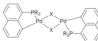
1a R = naphthyl, X = OAc 1b R = naphthyl, X = I 1c R = naphthyl, X = Br
