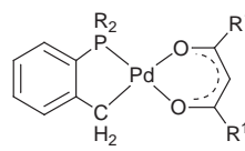
3a R = o -tolyl, R 1 = Me 3b R = o -tolyl, R 1 = CF 3
