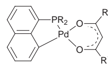
2a R = naphthyl, R 1 = Me 2b R = naphthyl, R 1 = CF 3
