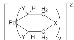
11a X = OC(=O)O 11b X = O
