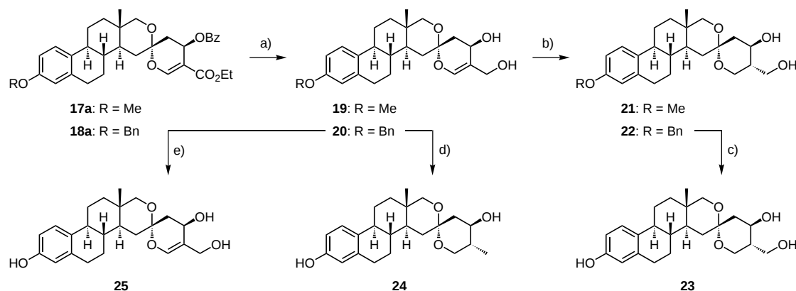
Scheme 3. Synthesis of the estrone–talaromycin hybrids 23 , 24 , and 25 ; a) 12 equiv DIBAH, THF/CH 2 Cl 2 , –78 °C, 21 h; 19 : 70 %; 20 : 76 %; b) 10 mol % PtO 2 , H 2 (50 bar), MeOH/ethyl acetate, RT, 12 h, 99 %; c) 10 mol % Pd/C, H 2 (65 bar), MeOH/ethyl acetate, RT, 20 h, 99 %; d) 10 mol % Pd/C, H 2 (65 bar), MeOH/ethyl acetate, RT, 24 h, 99 %; e) Li, NH 3 (l), MeOH, –78 °C, 3 h, 90 %.
