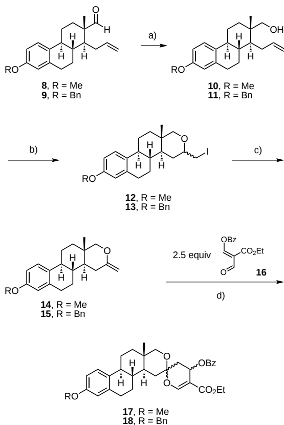
Scheme 2. Synthesis of the spiroacetals 17 and 18 ; a) 8 : 10 equiv NaBH 4 , MeOH, RT, 30 min; 9 : 10 equiv KBH 4 , MeOH, RT, 30 min, 99 % of 11 ; b) I 2 , NaHCO 3 , Et 2 O/H 2 O, RT, 4 h; 12 : 99 % from 8 ( ds = 2:1); 13 : 96 % ( ds = 2.5:1); c) DBU (neat), 90–100 °C, 30 min; d) toluene/CH 2 Cl 2 , RT, 14 h; 17 : 76 % from 12 ( dr = a:b:c:d = 3.9:3.2:1.0:1.0); 18 : 72 % from 13 ( dr = a:b:c:d = 4.5:4.0:1.5:1.0); Bn = benzyl, Bz = benzoyl.
