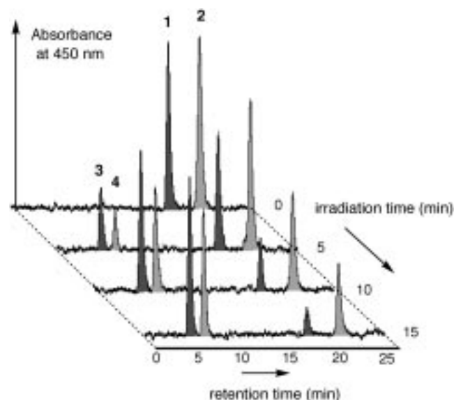
Figure 2. Series of reversed-phase HPLC chromatograms obtained during the light induced conversion of the model compounds 1 and 2 into the cleaved products 3 and 4 (ethylene glycol). The chromatograms show 1 and 2 eluting at approximately 18 min and 21 min, respectively. The cleavage products 3 and 4 elute at approximately 6 min and 8 min, respectively. Conditions: Lichrosphere column (250 × 4) 100/5. Gradient: water/methanol from 70:30 to 10:90 over 30 min. Detection at 450 nm.
