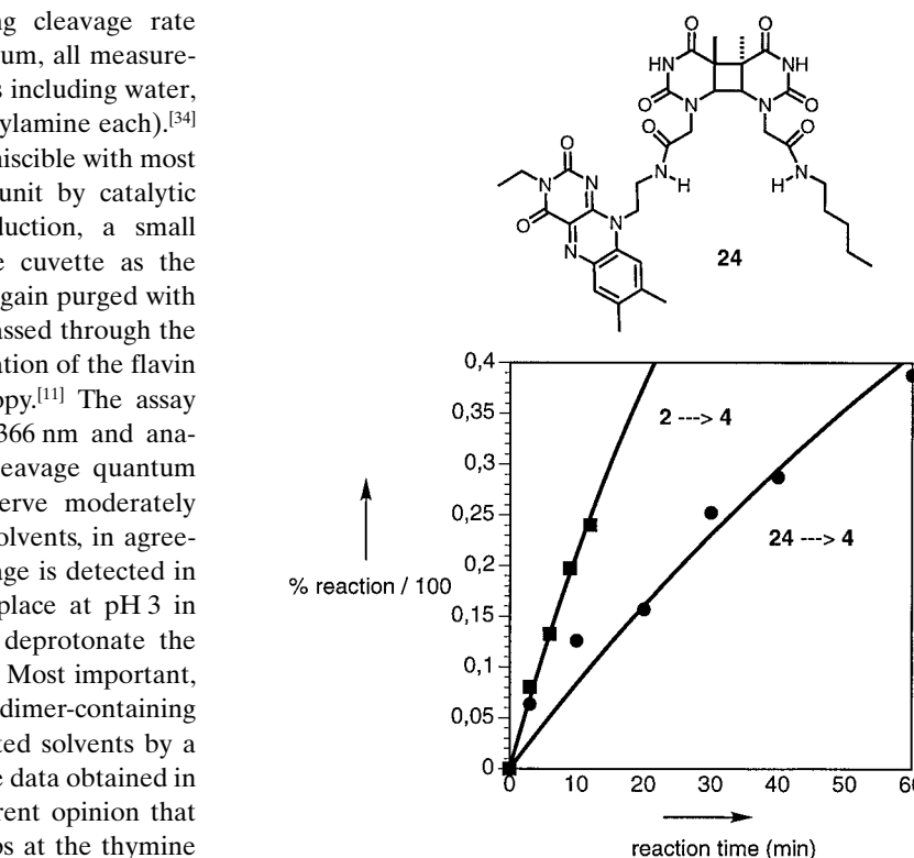
Figure 5. Time-dependent formation of the cleaved photoproduct 4 during the irradiation of 2 and 24 . Irradiation was performed at \lambda = 366 nm in ethylene glycol at 25^\circ\text{C} . ■: 4 formed upon irradiation of 2 . ●: 4 formed upon irradiation of 24 .
