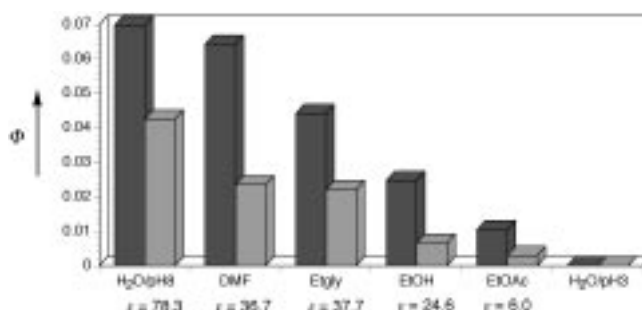
Figure 4. Bar diagrams showing the quantum yields ( \Phi ) for the cleavage process of 1 and 2 reacting to 3 and 4 in various solvents. DMF = dimethylformamide, Etgly = ethylene glycol, EtOH = ethanol, EtOAc = ethyl acetate. Irradiation was performed at \lambda = 366 \text{ nm} at 25 °C. Dark grey bars: uracil model compound 1 . Light grey bars: thymine model compound 2 .
