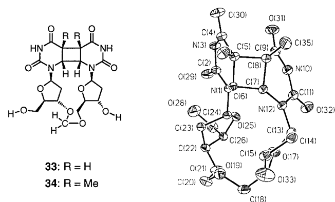
Figure 6. Depiction of the molecular structures of the uridine and thymidine photodimer analogues 33 and 34 used for the enzymatic studies. X-ray crystal structure of the thymidine dimer 34 . For the crystal structure of 33 see ref. [21]. ORTEP plot of the molecular structure. Arbitrary numbering. Displacement ellipsoids are shown at the 50% probability level.
