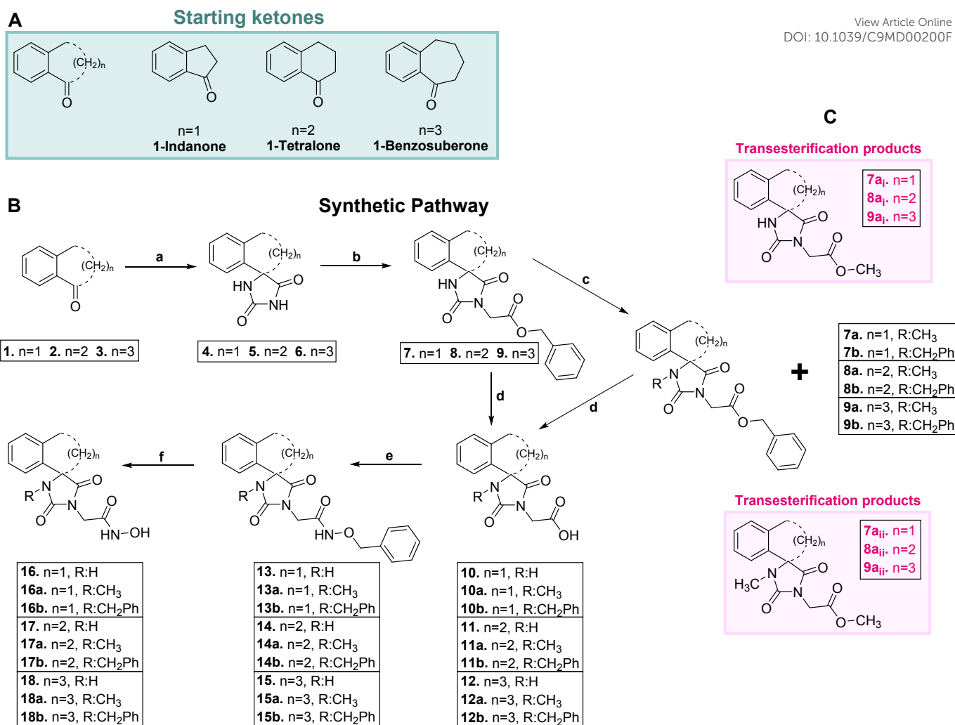
Scheme 1 A) Starting ketones B) Synthesis of the target acetohydroxamic acid analogues 16-18 , 16a-18a and 16b-18b . Reagents and Conditions: (a) Method A: NaCN (2.27 eq), (NH 4 ) 2 CO 3 (6 eq), EtOH/H 2 O (1.1:1), reflux, 8 h - 11 days; | Method B: KCN (1.3 eq), (NH 4 ) 2 CO 3 (5 eq), EtOH/H 2 O (1:3), MW (100 W), 120 °C, 25 min - 1 h; (b) (i) [(CH 3 ) 3 Si] 2 NK (1.02 eq), dry THF (0-5 °C) and then r.t., 20 min - 1 h, Argon; (ii) BrCH 2 COOCH 2 Ph (1.05 eq), dry DMF, 35-38 °C, 48 h, Argon; (c) (i) NaH (1.2 eq), dry DMF, (0-5 °C) and then r.t., 15 min, Argon; (ii) PhCH 2 Br (1.2 eq), 60 °C, 7 days, Argon; (d) H 2 , Pd/C 10%, EtOH/AcOEt 3:1, 50-55 psi, 40-45 °C, 3h; (e) Method A: EDCI·HCl (1.2 eq), HOBt (1.2 eq), PhCH 2 ONH 2 ·HCl (1.2 eq), TEA (5.8 eq), dry CH 2 Cl 2 /dry DMF, 30-35 °C, 40 h, Argon; | Method B: (i) CDI (1.2 eq), dry THF, 28-30 °C, 1 h, Argon; (ii) PhCH 2 ONH 2 ·HCl (1.2 eq), TEA (1.82 eq), 28-30 °C, 24 h, Argon; (f) H 2 , Pd/C 10%, EtOH/AcOEt 3:1, 50-55 psi, 40-45 °C, 3h. C) Methyl esters obtained because of unexpected transesterification reaction (pink frames).
