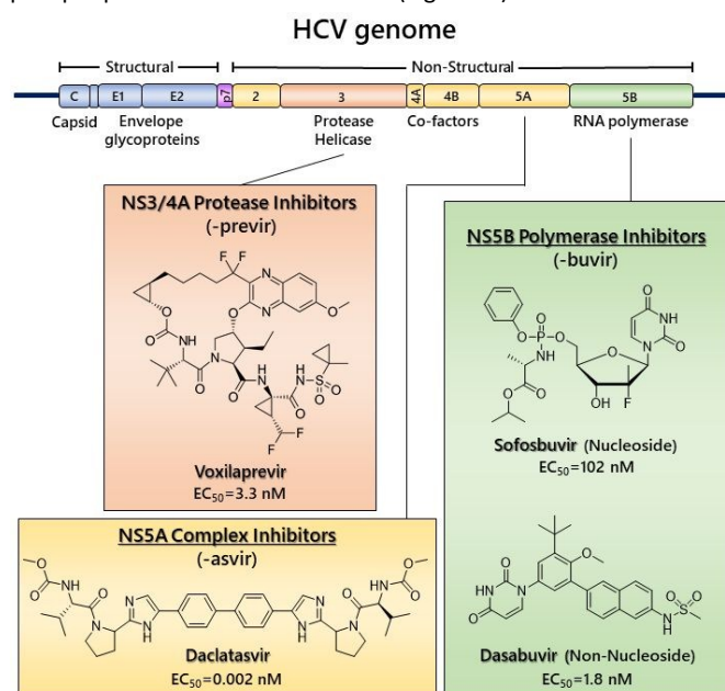
Figure 1 Representative chemical structures of clinically approved DAAs and their respective \text{EC}_{50} s against HCV genotype 1b.
