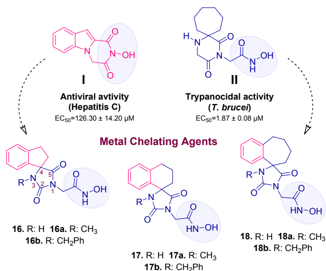
Figure 3 Indole-flutimide analogue (I) with antiviral activity, cycloheptane spiro-substituted 2,6-DKP analogue (II) with trypanocidal activity and novel synthesized analogues reported in this study. Metal binding groups are indicated in plum elliptical shape.
