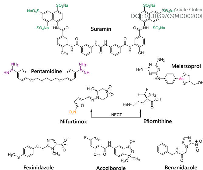
Figure 2 Currently available marketed drugs for treatment of HAT and Chagas disease. Highlighted regions are reported to play a major role in the mechanism of action. Chemical structures of potential drug candidates Fexinidazole and Acoziborole.
