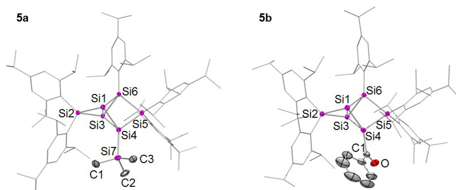
Figure 1. Structures of 5a,b in the solid state (thermal ellipsoids at 50% probability). Hydrogen atoms and co-crystallized pentane omitted. a: E = SiMe 3 , b: E = COPh.
