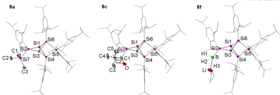
Figure 3. Structures of 6a , 6c and 6f in the solid state (thermal ellipsoids at 50% probability). Hydrogen atoms and co-crystallized solvent molecules omitted. a: E = TMS, c: E = CO t Bu, f: E = BH 3 − .
