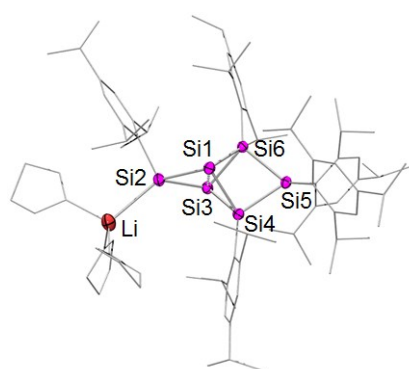
Figure 2: Structure of 4Li in the solid state (thermal ellipsoids at 50% probability). Hydrogen atoms and co-crystallized solvent molecules omitted.
