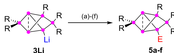
Scheme 2: Synthesis of ligato -functionalized siliconoids 5a-f. Reagents: a) Me 3 SiCl, b) PhCOCl, c) t BuCOCl, d) ClP(NMe 2 ) 2 , e) SiCl 4 , f) BH 3 ·SMe 2 . 5a: E = Me 3 Si, 5b: E = COPh and the previously reported 32 5c: E = CO t Bu, 5d: E = P(NMe 2 ) 2 , 5e: E = SiCl 3 , 5f: E = BH 3 – .
