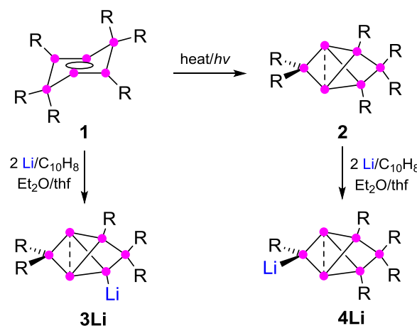
Scheme 1: Synthesis of 3Li 32 and 4Li (this work) from dismutational hexasilabenzene isomer 1 and from the global minimum isomer 2 (Tip = 2,4,6-triisopropylphenyl).
