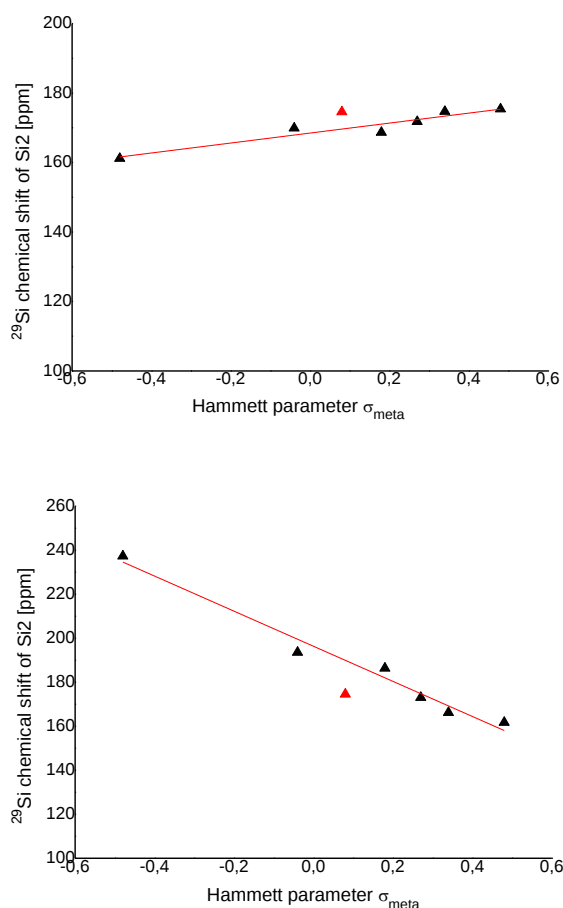
Figure 4. Plots of the Hammett parameters \sigma_m vs. ^{29}\text{Si} chemical shifts of the privo silicon vertices of ligato ( 5a-f ; top) and privo functionalized hexasilabenzpolarenes ( 6a-f ; bottom). The data pair marked with red triangles corresponds to the unfunctionalized hexaaryl derivative 2 .
