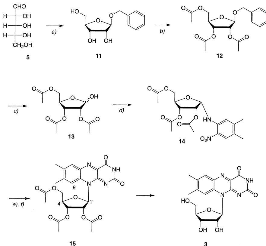
Scheme 2. Synthesis of the Flavin \beta -D-Ribofuranoside 15 and Attempts to Deprotect 15 to Give 3
