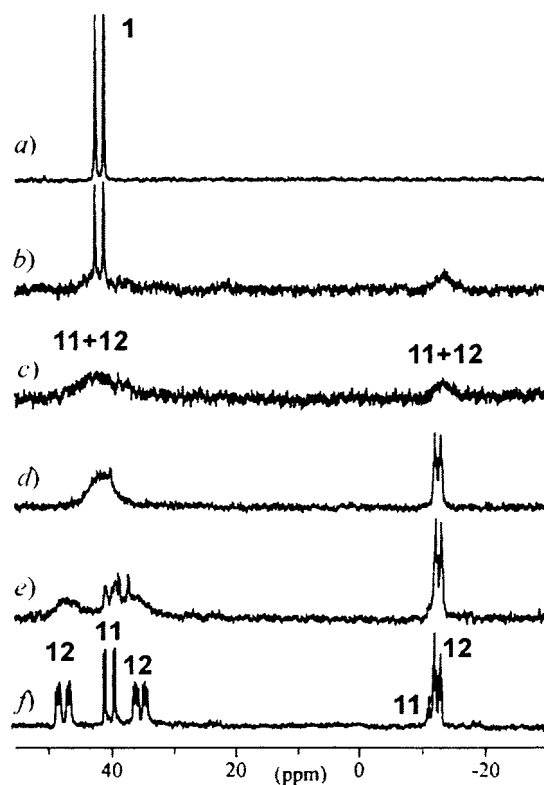
Fig. 2. ^{31}\text{P}\{^1\text{H}\} -HP-NMR Study (sapphire tube, (\text{D}_8)\text{THF} , 81.01 MHz) of the hydrogenation of 1 in the presence of TfOH ( \text{TfOH}/\mathbf{1} 3:1). a) At r.t. and ambient pressure, b) under 30 bar \text{H}_2 for 20 min at r.t., c) after heating 60 min at 40^\circ , d) after cooling to r.t., e) to 0^\circ , and f) to -30^\circ .
