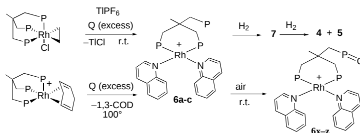
Scheme 7
