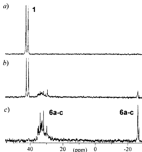
Fig. 3. ^{31}\text{P}\{^1\text{H}\} -HP-NMR Study (sapphire tube, (\text{D}_8) THF, 81.01 MHz) of the catalytic hydrogenation of Q in the presence of 1 and TfOH ( Q / TfOH / 1 40:10:1). a ) at r.t. and ambient pressure, b ) pressurized to 30 bar with \text{H}_2 for 15 min at r.t., and c ) after heating to 40^\circ for 60 min.
