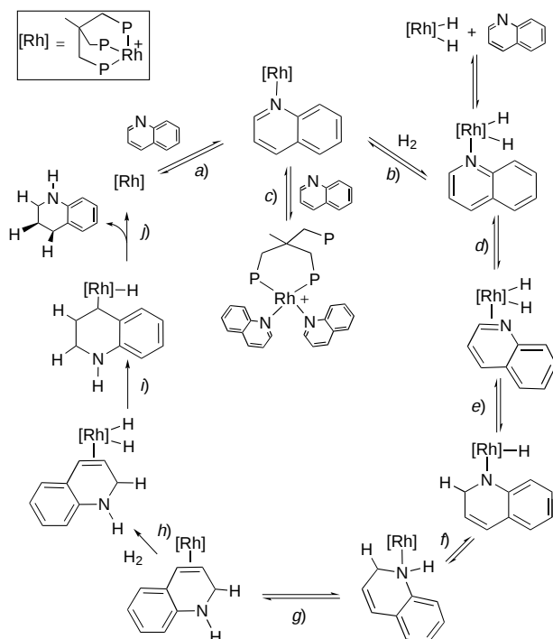
Scheme 11
