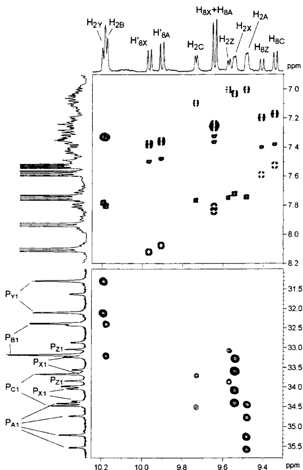
Fig. 5. Section of the ^1\text{H} -TOCSY spectrum (upper) and 2D ^1\text{H} - ^{31}\text{P} correlation (lower) of the 6a – c/6x – z mixture (500.13 MHz, ( \text{D}_8 )THF, 21 ^\circ )
