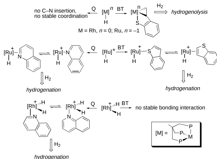
Scheme 12
