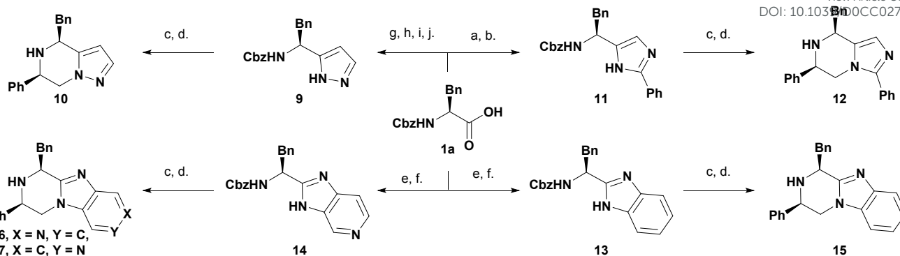
Scheme 2: A: Synthesis of other bicyclic scaffolds: a. 2-aminoacetophenone hydrochloride, EDC, HOBT, NMM, DCM, 3h, 0 °C to rt; b. \text{NH}_4\text{OAc} , xylene, 8h, reflux; c. 2-bromoacetophenone, \text{K}_2\text{CO}_3 , acetone, 12h, rt; d. \text{NH}_4\text{CO}_2\text{H} , \text{Pd}(\text{OH})_2/\text{C} (20 mol %), \text{MeOH}:\text{H}_2\text{O} (3:1 v/v), 12h, rt; e. o-phenylenediamine or 3,4-diaminopyridine, HATU, DIPEA, DCM, 12h, rt; f. AcOH 2h, 40 °C; g. \text{HNMeOMe}\cdot\text{HCl} , HOBT, HBTU, DIPEA, DCM, 12h, rt; h. phenylethylene magnesium bromide, THF, 12h, -78 °C to rt; i. \text{HNEt}_2 , DCM, 12h, rt; \text{N}_2\text{H}_4\cdot\text{H}_2\text{O} , HCl, 3h, reflux (see SI for yields).
