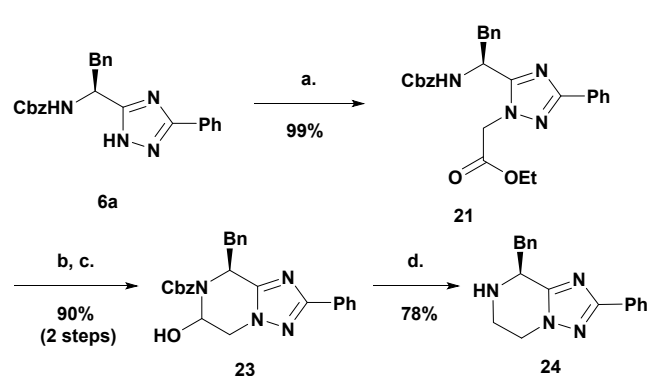
Scheme 4: Synthesis of scaffold with a single chiral centre in the \text{R}_2 -position: a. ethyl-2-bromoacetate, \text{K}_2\text{CO}_3 , 12h, rt; b. \text{LiBH}_4 , \text{Et}_2\text{O} , 3h, 0 °C to rt; c. IBX, \text{EtOAc} , 12h, reflux; d. \text{NH}_4\text{CO}_2\text{H} , \text{Pd}(\text{OH})_2/\text{C} (20 mol %), \text{MeOH}:\text{H}_2\text{O} (3:1 v/v), 12h, rt.
