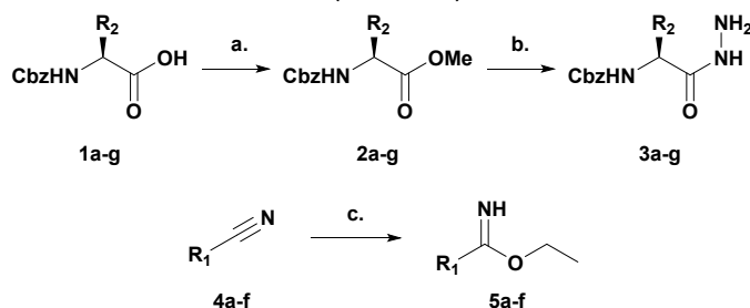
Scheme 1: Building block synthesis (see Table 1 for R_1 and R_2 ): a. \text{SOCl}_2 , MeOH, 3h, rt, 96–100%; b. \text{NH}_2\text{NH}_2 \cdot \text{H}_2\text{O} , MeOH, 12h, rt, 82–100%; c. \text{AcCl} , EtOH, 12h, 0 °C to rt, 66–100%.
