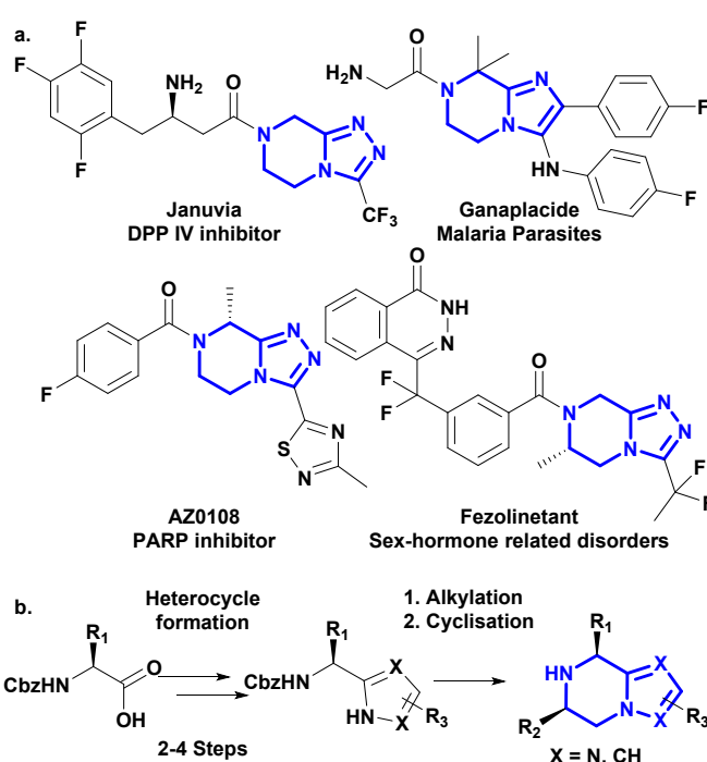
Figure 1: a. Fused piperazine scaffolds (highlighted in blue) utilised in FDA approved drugs and clinical candidates; 6 b. Synthetic strategy developed in this work to access these fused piperazine scaffolds.
