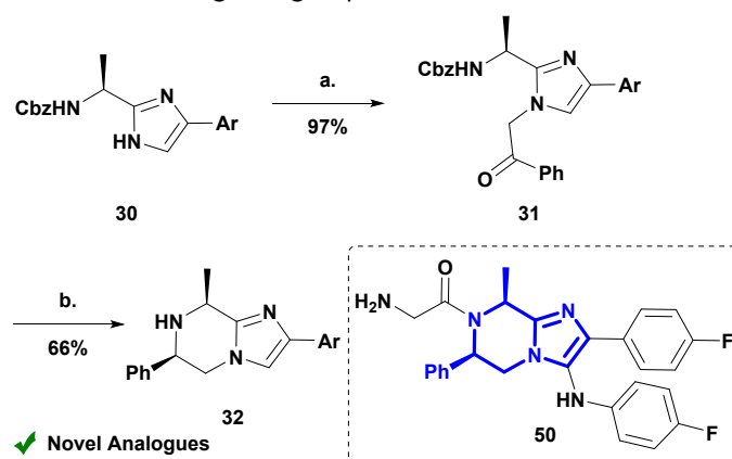
Scheme 5: Synthesis of ganaplacide analogue intermediate (full synthetic route for ganaplacide and analogue in the SI): a. 2-bromoacetophenone, \text{K}_2\text{CO}_3 , acetone, 97%; b. \text{NH}_4\text{CO}_2\text{H} , \text{Pd}(\text{OH})_2/\text{C} (20 mol %), \text{MeOH}:\text{H}_2\text{O} (3:1 v/v), 66%. Ar = p -PhF
