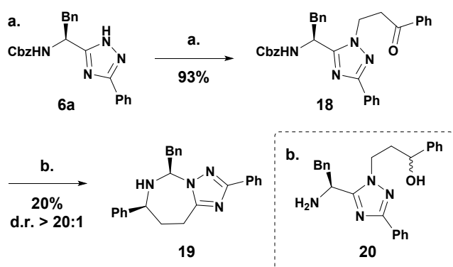
Scheme 3: a: Synthesis of exemplar 5,7-bicyclic scaffold. a. 3-chloropropiophenone, \text{K}_2\text{CO}_3 , acetone, 12h, rt; b. \text{NH}_4\text{CO}_2\text{H} , \text{Pd}(\text{OH})_2/\text{C} (20 mol %), \text{MeOH}:\text{H}_2\text{O} (3:1 v/v), 12h, rt. b. Undesired side product 20 .
