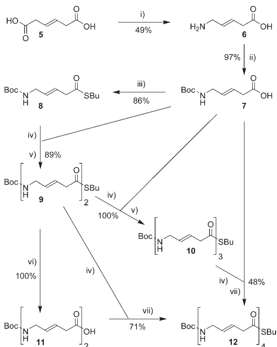
Scheme 1. Preparation of thioester precursors 8–10 and 12 . i) \text{H}_2\text{SO}_4 , \text{NaN}_3 , \text{CHCl}_3 , 45^\circ\text{C} ; ii) \text{Boc}_2\text{O} , \text{NaOH} , t BuOH, \text{H}_2\text{O} , RT; iii) n BuSH, EDCI, DMAP, HOBt, \text{CH}_2\text{Cl}_2 , -17^\circ\text{C} ; iv) TFA, \text{CH}_2\text{Cl}_2 , RT; v) DCC, DMAP, NMM, \text{CH}_2\text{Cl}_2 , 0^\circ\text{C} ; vi) KOH, \text{H}_2\text{O} , MeOH, RT; vii) DCC, DMAP, NMM, EtOAc, 0^\circ\text{C} .
