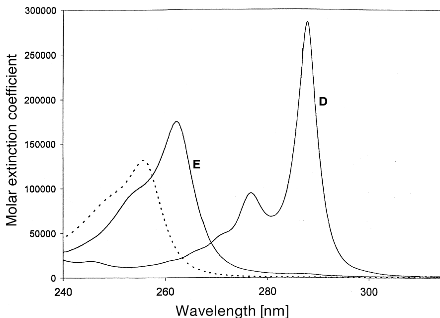
Fig. 4. Absorption spectra ( S_0 \rightarrow S_2 electronic transition) of anthracene (····) and probes D and E in \text{CHCl}_3
