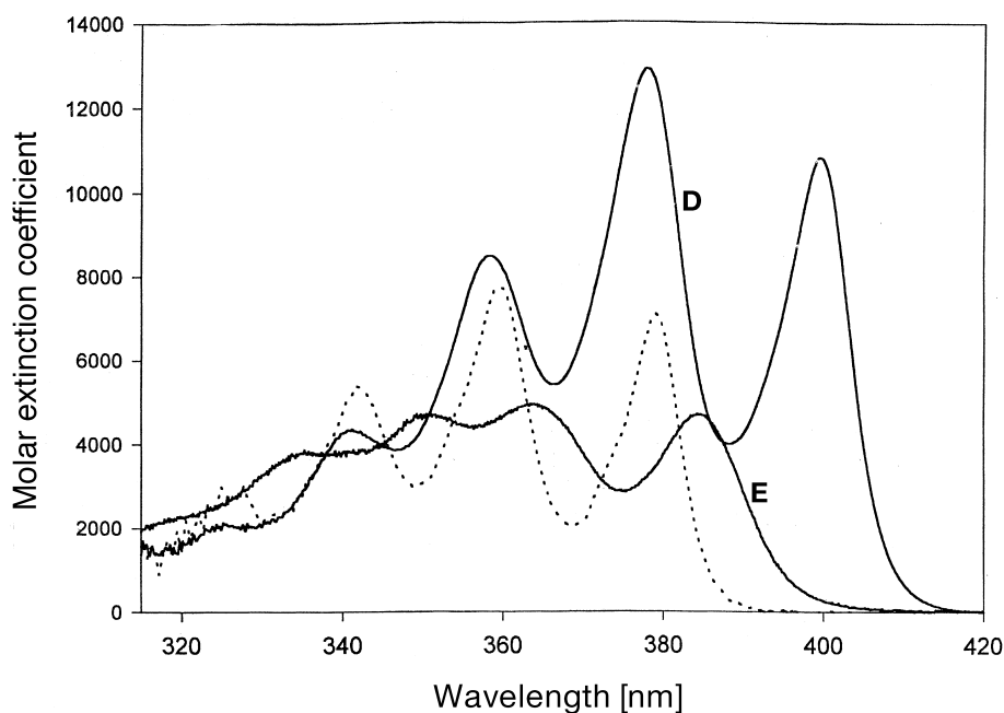
Fig. 3. Absorption spectra ( S_0 \rightarrow S_1 electronic transition) of anthracene (····) and probes D and E in \text{CHCl}_3
