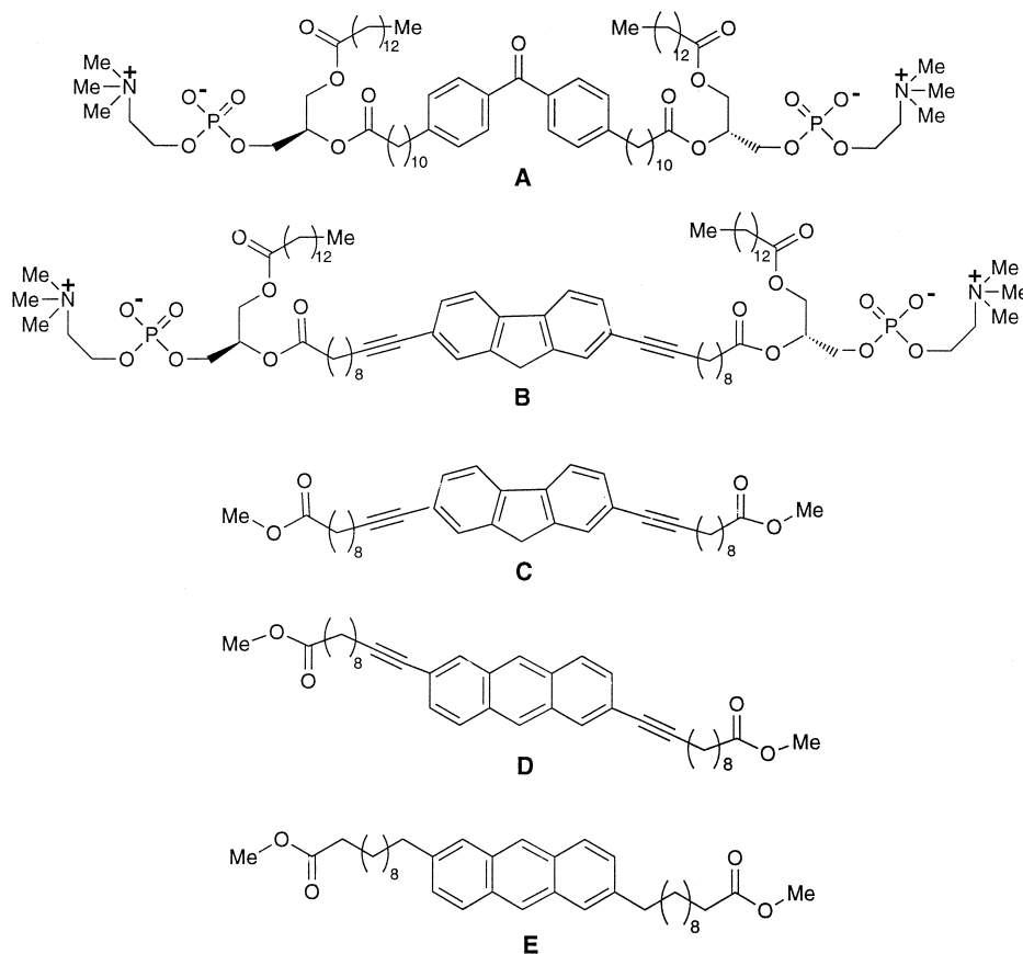
Fig. 1. Structure of transmembrane photosensitive or fluorescent probes
