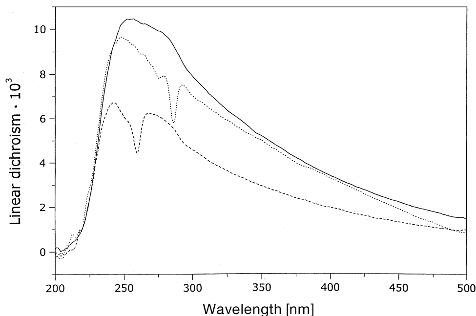
Fig. 7. Linear dichroism (LD) of shear-deformed DMPC vesicles at 35^\circ and 3100\text{ s}^{-1} : DMPC vesicles (—), DMPC vesicles with probe E (····) and DMPC vesicles with probe D (---). Probe/lipid ratio 1:100. The blank DMPC vesicles exhibit strong scattering with increasing positive LD when passing from 500 to 250 nm; the negative LD at shorter wavelength is due to lipid absorption. The two peaks at 285 and 260 nm show that their anthracenediyl long axes are preferentially oriented along the lipid chains (for theory of interpretation of shear LD of liposomes, see [14]).
