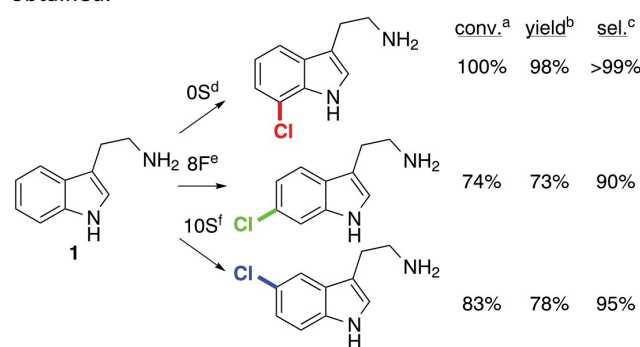
Figure 4. Chlorination of tryptamine using engineered halogenases. a Conversion of starting material determined by UPLC analysis of crude reaction mixtures. b Isolated yield of pure product. c Selectivity determined by NMR analysis of a purified mixture of isomers (inseparable by preparative chromatography). d 10 μM 0S, 0.5 mM tryptamine (10 mg), 2.5 μM MBP-RebF, 9 U/mL GDH, 10 mM NaCl, 20 mM glucose, 100 μM NAD and FAD, 0.5% v/v i -PrOH/25 mM HEPES buffer, pH 7.4, 25 °C. e As in (d) but 50 μM 8F, 16 °C. f As in (d) but 50 μM 10S, 100 mM NaCl, 10 °C.
