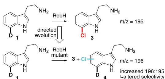
Figure 2. Mass spectrometry assay for halogenase selectivity using probe substrate 1 .
