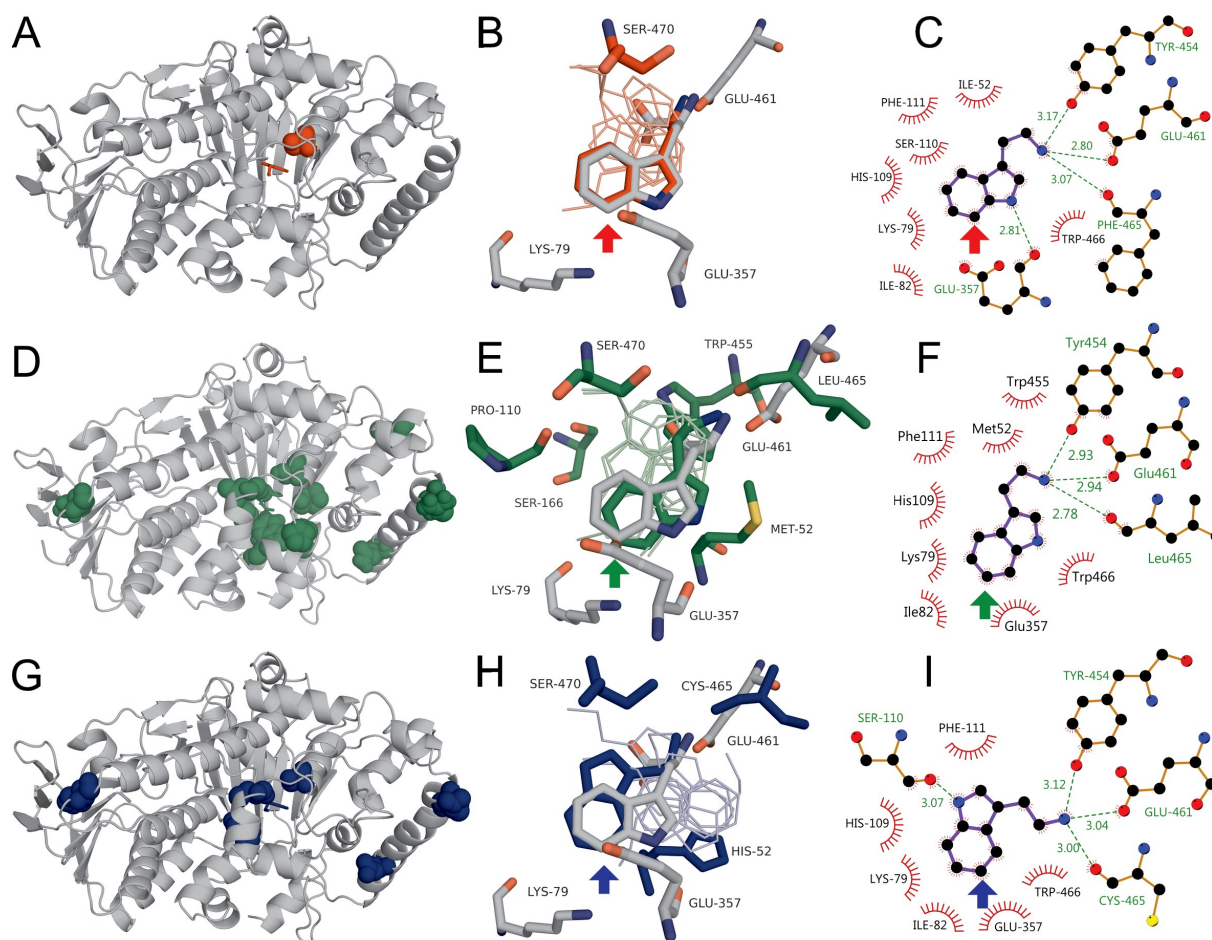
Figure 6. Location of mutations and tryptamine poses for 0S (red), 8F (green), and 10S (blue) mapped onto the RebH structure (grey). A, D, and G) Location of mutations (spheres) and tryptamine poses (sticks). B, E, and H) Active site mutations, conserved residues, tryptamine poses consistent with observed selectivity, and native tryptophan pose (sticks) and additional tryptamine poses (lines). C, F, and I) Binding interactions in poses consistent with observed selectivity. Colored arrows indicate the chlorination site. 61
