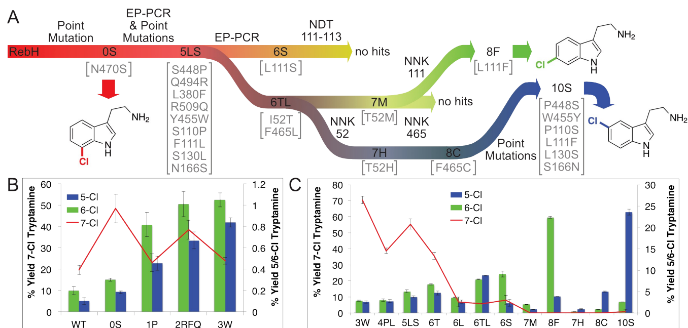
Figure 3. A) Lineage diagram showing mutagenesis methods and mutations found in selected variants above and below the lineage arrows, respectively. B/C) Yield of 7- (left y-axis) and 6- and 5-chlorotryptamine (right y-axis) for different variants along the halogenase lineage. Reactions conducted using 2.5 \mu M MBP-RebF, 9 U/mL GDH, 100 mM NaCl, 20 mM glucose, 100 \mu M NAD and FAD, 0.5 mM phenol, 0.5% v/v i -PrOH/25 mM HEPES buffer, pH 7.4, 25 ^{\circ} C. Substrate and enzyme concentrations: B) 1.5 mM 2 , 15 \mu M RebH variant. C) 0.5 mM 2 , 25 \mu M RebH variant.
