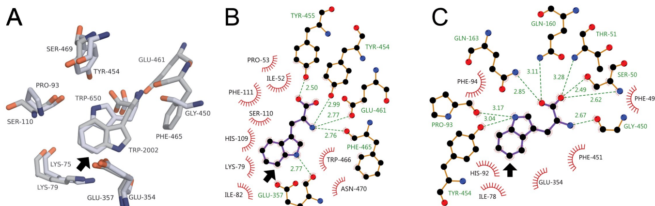
Figure 5. A) Key residues in the RebH (grey carbons) and PyrH (light blue carbons) active sites. Interactions involved in tryptophan binding in B) RebH and C) PyrH. Arrow denotes chlorination site.
