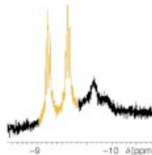
Figure 2. Hydride region of the ^1\text{H} NMR spectrum of [\text{HRh}(\text{L})(\text{CO})_2] , \text{L} = \mathbf{6a} .
