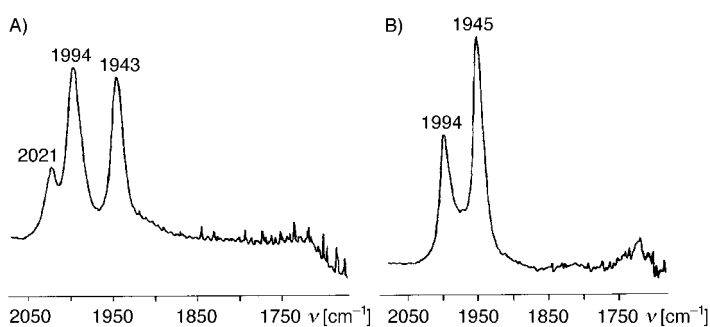
Figure 3. In situ IR spectrum of [\text{HRh}(\text{L})(\text{CO})_2] , \text{L} = \mathbf{6a} ( \text{L}:\text{Rh} = 2:1 ), 323 K. A) 20 bar ( \text{CO:H}_2 = 1:1 ). B) 20 bar ( \text{CO:D}_2 = 1:1 ).
