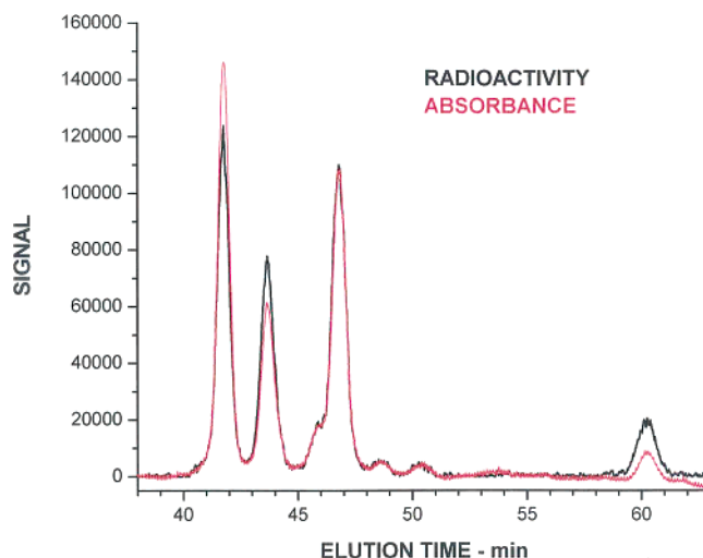
Figure 5. Comparison of radiochromatographic and spectrophotometric recordings (at 265 nm) for 2,3-dimethylbutane containing 1 mM ^{125}\text{I}_2 irradiated to a dose of 100 krad. Elution was with 40:60 hexane–isopentane. The isopropyl iodide peak at 46.8 min was used to normalize the chromatograms.
