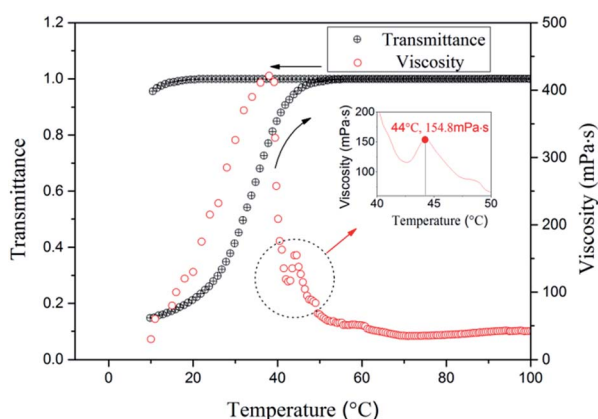
Fig. 3 The transmittance and viscosity (rheological behaviors; the shear rate is 1 s -1 ) of the 1% GAS solution.
