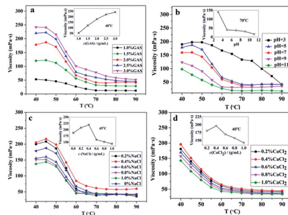
Fig. 4 The apparent viscosities (shear rate: 50 s -1 ) versus temperature for (a) different GAS concentrations, (b) different pH, (c) different NaCl concentrations, w(GAS) = 2%, and (d) different CaCl 2 concentrations, w(GAS) = 2%.
