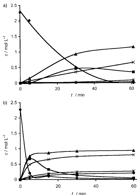
Figure 4. Kinetics of the hydroformylation of oct-1-ene with [\text{Rh}(\text{CO})_2\text{acac}]/\mathbf{8} , in toluene ( c_0 = 2.27 \text{ M} ) (oct-1-ene/ \mathbf{8}/\text{Rh} , 4166:20:1) at a) 90 °C, 10 bar ( \text{CO}/\text{H}_2 1:1) and b) 130 °C, 40 bar ( \text{CO}/\text{H}_2 1:1); \blacklozenge = oct-1-ene, \blacksquare = internal octene isomers, \blacktriangle = n -nonanal, \times = 2-methyl octanal, * = 2-ethylheptanal.
