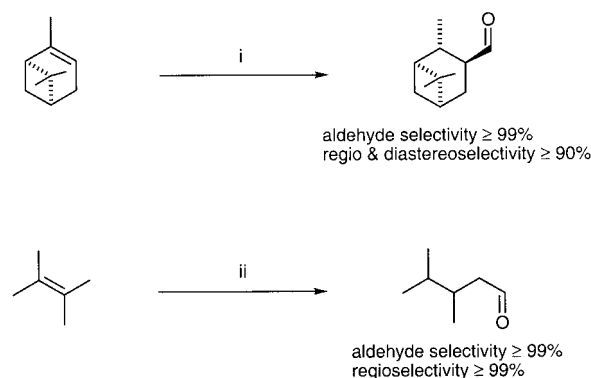
Scheme 10. Hydroformylation of tri- and tetrasubstituted alkenes. i) \text{Rh}/\mathbf{8} , \text{CO}/\text{H}_2 , 60 bar, T = 80^\circ\text{C} , toluene. TOF = 56 \text{ h}^{-1} . ii) \text{Rh}/\text{L} , \text{CO}/\text{H}_2 , 60 bar, T = 100^\circ\text{C} , toluene. TOF [\text{h}^{-1}] \text{L} = \text{PPh}_3 : < 1, \text{L} = \mathbf{8} : 118.
