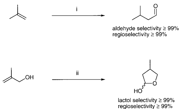
Scheme 9. Hydroformylation of 1,1-disubstituted alkenes. i) \text{Rh}/\text{L} , \text{CO}/\text{H}_2 , 30 bar, T = 80^\circ\text{C} , toluene. TOF [\text{h}^{-1}] \text{L} = \text{PPh}_3 : 332, \text{L} = \mathbf{8} : 3132. ii) \text{Rh}/\text{L} , \text{CO}/\text{H}_2 , 20 bar, T = 90^\circ\text{C} , toluene. TOF [\text{h}^{-1}] \text{L} = \text{PPh}_3 : 1317, \text{L} = \mathbf{8} : 3291.
