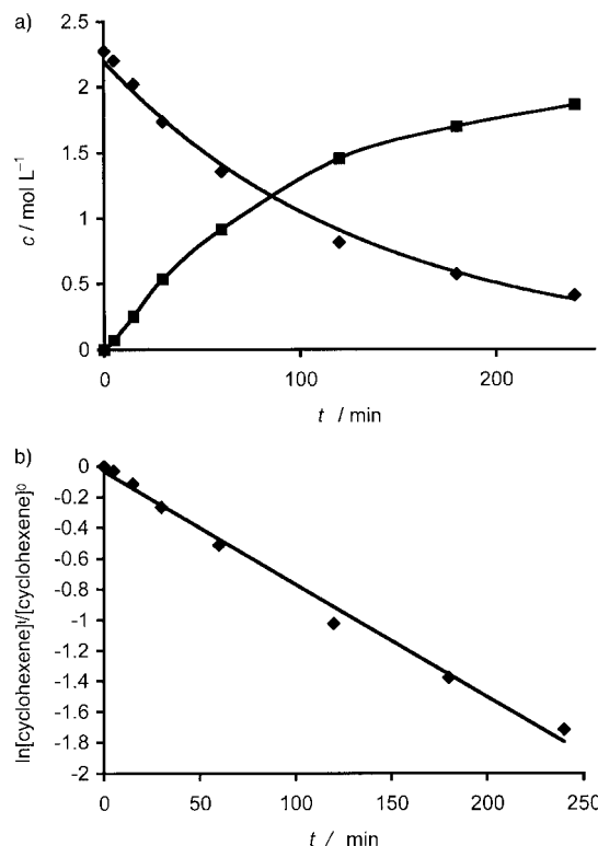
Figure 5. a) Kinetics of the hydroformylation of cyclohexene with phosphine 8 / [\text{Rh}(\text{CO})_2\text{acac}] at 90 °C, 40 bar in toluene ( c_0 = 2.63 \text{ M} ) for 4 h (cyclohexene/ \text{L}/\text{Rh} , 4166:20:1), \blacktriangle c(\text{cyclohexene}) , \blacksquare c(\text{cyclohexanecarbaldehyde}) ; b) Logarithmic plot of cyclohexene concentration against time ( k_{\text{hydroform.}} = 7.3 \times 10^{-3} \text{ s}^{-1} ).
