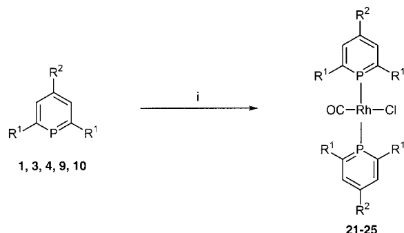
Scheme 6. Preparation of trans -[(phosphinine) _2\text{RhCl}(\text{CO}) ] complexes 21–25 . i) [\text{Rh}(\text{CO})_2\text{Cl}]_2 , \text{CH}_2\text{Cl}_2 , RT, 30 min, (quant.). 21 : \text{R}^1 = \text{Me} , \text{R}^2 = \text{Ph} ; 22 : \text{R}^1 = \text{Ph} , \text{R}^2 = \text{Ph} ; 23 : \text{R}^1 = 2\text{-Naphth} , \text{R}^2 = \text{Ph} ; 24 : \text{R}^1 = \text{Ph} , \text{R}^2 = \text{C}_6\text{H}_4(p\text{-OMe}) ; 25 : \text{R}^1 = \text{Ph} , \text{R}^2 = \text{C}_6\text{H}_4(p\text{-CF}_3) .
