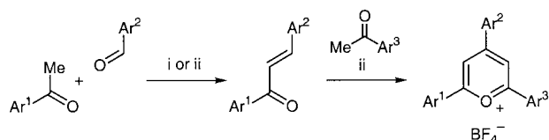
Scheme 3. i) 10 mol % \text{Ba}(\text{OH})_2 , ethanol, 20–80 °C; ii) \text{HBF}_4 (52 % ethereal solution), 1,2-dichloroethane, reflux, 4 h (22–62 %).
