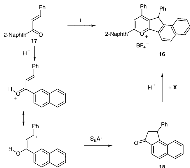
Scheme 4. i) \text{HBF}_4 (52 % ethereal solution), 1,2-dichloroethane, reflux, 4 h (28 %).
