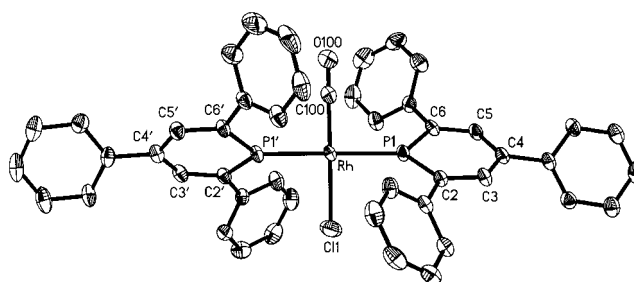
Figure 1. Ortep plot of the structure of trans -[( 3 ) _2\text{RhCl}(\text{CO}) ] ( 22 ) in the solid state.
