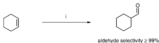
Scheme 8. Hydroformylation of cyclohexene. i) \text{Rh}/\text{L} , \text{CO}/\text{H}_2 , 40 bar, T = 90^\circ\text{C} , toluene. TOF [ \text{h}^{-1} ] \text{L} = \text{PPh}_3 : 109, \text{L} = \mathbf{8} : 1959.
