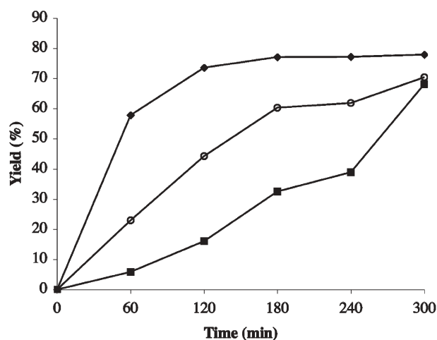
Fig. 1 Rates of formation of 4 in Scheme 4. Solvent systems: \blacklozenge \text{CH}_2\text{Cl}_2 -perfluoro(2-butyltetrahydrofuran) (4 mL/2 mL); \circ \text{CH}_2\text{Cl}_2 - \text{CF}_3\text{C}_6\text{F}_{11} (4 mL/2 mL); \blacksquare \text{CH}_2\text{Cl}_2 only (4 mL).
