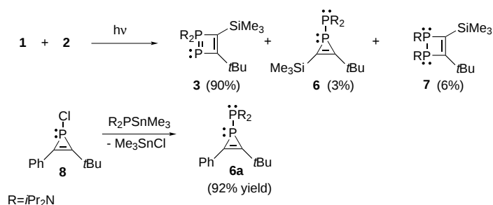
Scheme 2. Reaction scheme for the preparation of 3 , 6 , 6a , and 7 .
