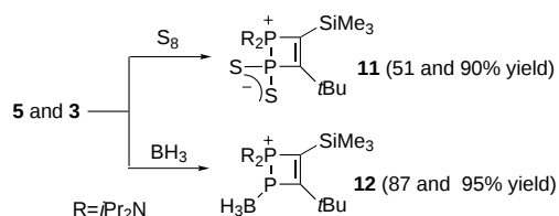
Scheme 7. Reaction scheme for the formation of 11 and 12 .
