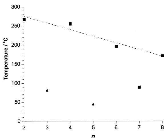
Figure 9. Measured melting temperatures (filled squares) for 2 , 4 , 6 , 7 and 8 and melting/decomposition temperatures (filled triangles) for 3 ·water and 5 ·(toluene) 2 . The melting/decomposition behaviour for 3 ·water and 5 ·(toluene) 2 is discussed fully in the text (the temperatures shown correspond to loss of solvent from these crystal structures).
