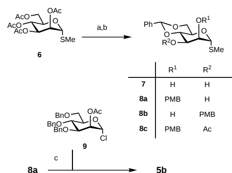
Scheme 2. Preparation of dimannosyl donor. a) \text{PhCH}(\text{OMe})_2 , CSA/DMF, 77 %; b) p\text{-MeOC}_6\text{H}_4\text{CH}_2\text{Cl} , \text{Bu}_4\text{NHSO}_4 , aq NaOH/ \text{CH}_2\text{Cl}_2 , 50 %; c) AgOTf, 2,6-di- tert -butyl-4-methylpyridine, MS 4 A/ \text{CH}_2\text{Cl}_2 , 81 %.
