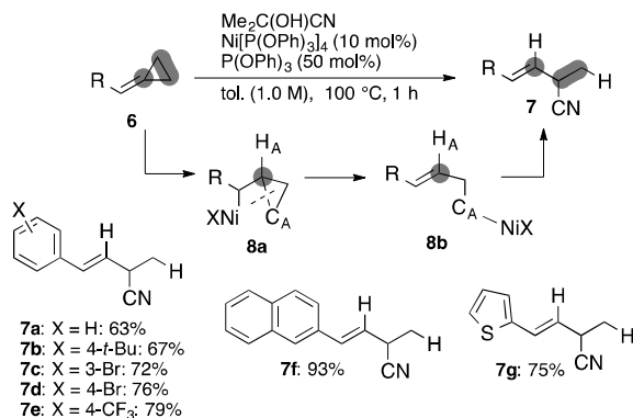
Scheme 8 Hydrocyanation of 6
