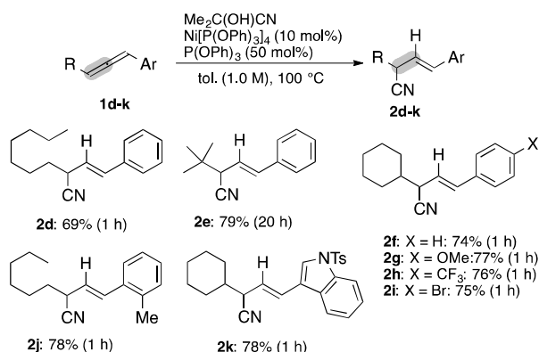
Scheme 3 Substrate scope of hydrocyanation using 1d-k
