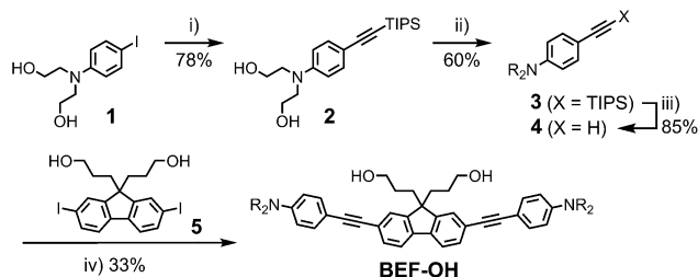
Scheme 1 Reagents: (i) TIPS-acetylene, \text{Pd}(\text{OAc})_2 , \text{PPh}_3 , \text{CuI} , DIPA, 50^\circ\text{C} , 16 h, (ii) \text{CH}_3(\text{OCH}_2\text{CH}_2)_6\text{OTs} , \text{NaH} , THF, reflux, 48 h, (iii) TBAF, THF, 20^\circ\text{C} , 12 h, (iv) 4 , \text{Pd}(\text{OAc})_2 , \text{PPh}_3 , \text{CuI} , DIPA, MeCN, 20^\circ\text{C} , 3 h; Ts = p -toluenesulfonate, TIPS = triisopropylsilyl, THF = tetrahydrofuran, DIPA = diisopropylamine, TBAF = tetra- n -butylammonium fluoride, R = (\text{CH}_2\text{CH}_2\text{O})_7\text{CH}_3 .
