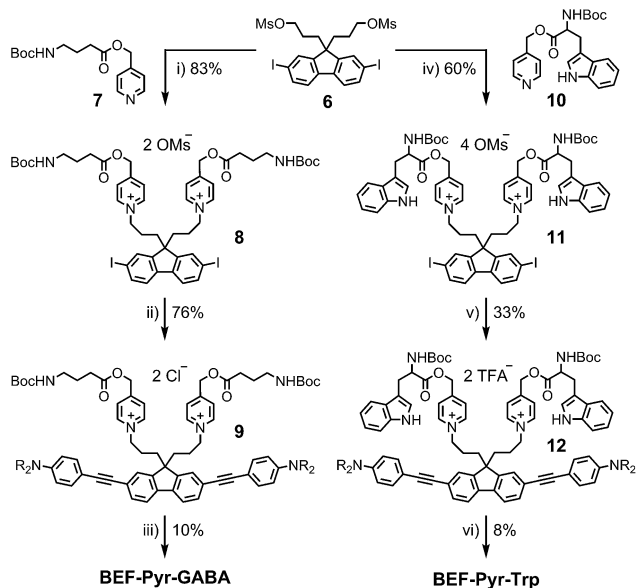
Scheme 2 Reagents: (i) MeCN, reflux, 36 h, (ii) 4 , \text{Pd}(\text{OAc})_2 , \text{PPh}_3 , \text{CuI} , DIPA, 20^\circ\text{C} , 1 h, brine wash, (iii) \text{BF}_3 \cdot \text{OEt}_2 , DCM, 0^\circ\text{C} \rightarrow 20^\circ\text{C} , 5 h, (iv) MeCN, 100^\circ\text{C} , 24 h, (v) 4 , \text{Pd}(\text{OAc})_2 , \text{PPh}_3 , \text{CuI} , DIPA, DCM, MeCN, 20^\circ\text{C} , 2 h, then purification in TFA-buffered solvent, (vi) \text{HCO}_2\text{H} , TIPS-H, 20^\circ\text{C} , 1 h.
