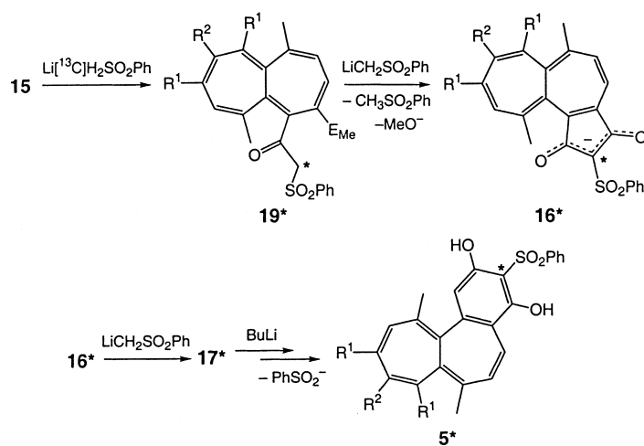
Scheme 8
