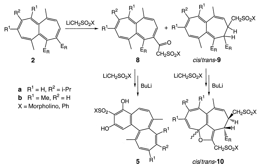
Scheme 2
