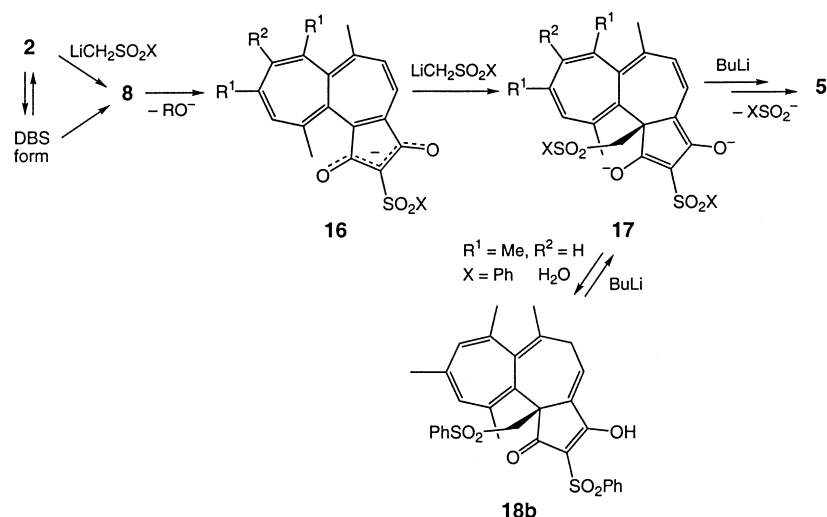
Scheme 7
