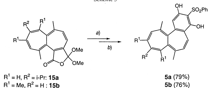
Scheme 5
