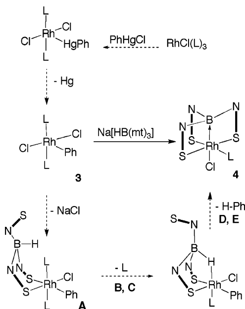
Scheme 1. Formation of the Rhodaboratranes 4 ( L = \text{PPh}_3 )
