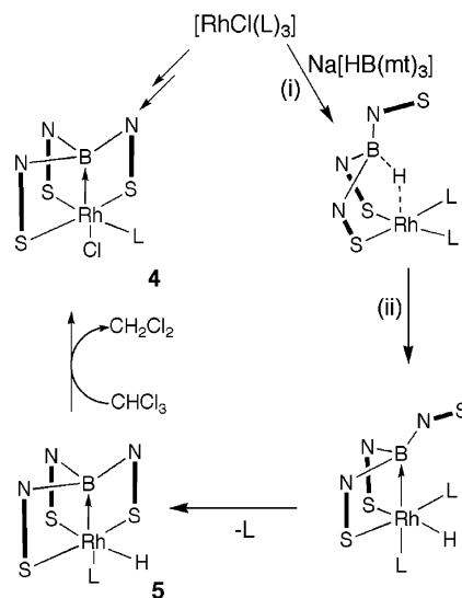
Scheme 2. Proposed Formation of the Rhodaboratrane 4 from Wilkinson's Catalyst ( \text{L} = \text{PPh}_3 )
