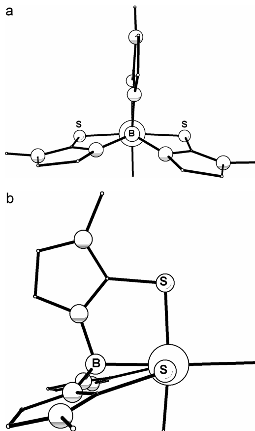
Figure 4. Projections of the simplified structure of 8 + along (a) B–Rh and (b) S1–S2 vectors illustrating distortion from local C 3v -B(mt) 3 Rh symmetry.
