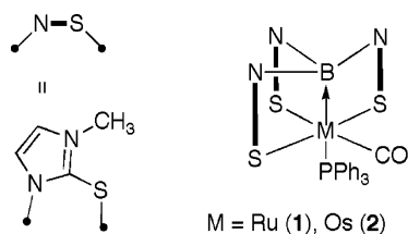
Chart 1. Metallaboratranes
