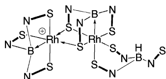
Chart 2. Dirhodaboratrane Cation in the Salt [\text{Rh}_2\{\text{B}(\text{mt})_3\}_2\{\kappa^2\text{-S,S}'\text{-HB}(\text{mt})_3\}]\text{Cl} ( 7 ·Cl)
