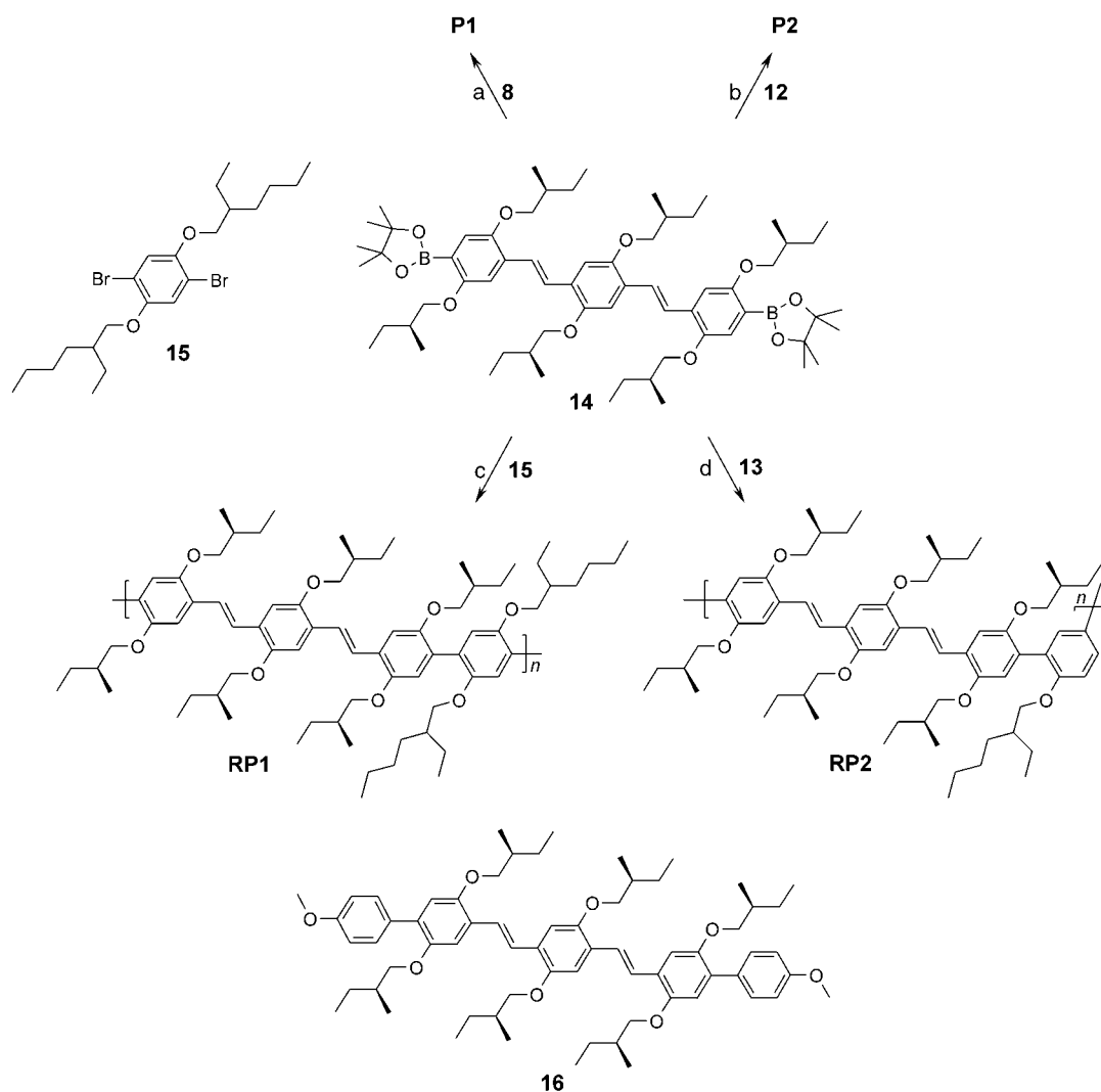
Scheme 4. Overview of the synthesis of the perylene bisimide-substituted polymers P1 and P2 , their reference polymers RP1 and RP2 , and the structure of model compound 16 . a) [\text{Pd}(\text{PPh}_3)_4] , \text{K}_2\text{CO}_3 , water, THF, 90^\circ\text{C} , 72%; b) [\text{Pd}(\text{PPh}_3)_4] , \text{K}_2\text{CO}_3 , water, THF, 90^\circ\text{C} , 75%; c) [\text{Pd}(\text{PPh}_3)_4] , \text{K}_2\text{CO}_3 , water, THF, 90^\circ\text{C} , 51%; d) [\text{Pd}(\text{PPh}_3)_4] , \text{K}_2\text{CO}_3 , water, THF, 90^\circ\text{C} , 55%.
