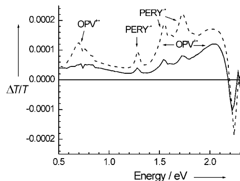
Figure 6. Near-steady-state photoinduced absorption spectra of P1 (—) and P2 (---) as thin films on quartz recorded at 80 K. The excitation wavelength is 458 nm, modulation frequency 275 Hz.
