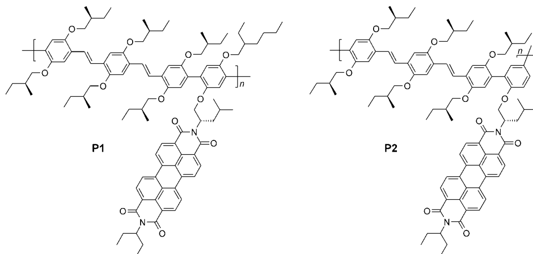
Scheme 1. Structures of donor-acceptor copolymers P1 and P2 .
