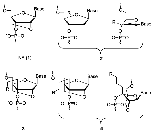
FIGURE 1. Constitution of LNA ( 1 ), 3'-C-branched-DNA ( 2 ), 3'-C-ethyl-LNA ( 3 ), and 3'-C-propyl-LNA ( 4 ) and a sketch of the S-type furanose conformation of monomer 2 and the N-type furanose ring conformation of monomers 3 and 4 .
