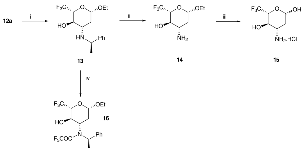
Scheme 2 Reagents and conditions: (i) BH 3 ·SMe 2 , CH 2 Cl 2 , 4 °C, 42 h then H 2 O 2 , 3 M NaOH, THF, MeOH (69% corrected); (ii) H 2 , 10% Pd on C, EtOAc, 17 h (100%); (iii) aqueous 0.5 M HCl, 100 °C (100%); (iv) TFAA, py then IRA 400 (OH) resin, MeOH (84%).
