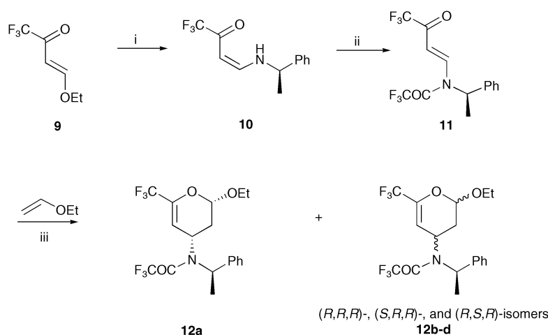
Scheme 1 Reagents and conditions: (i) (R) - \alpha -methylbenzylamine; CH 2 Cl 2 , 0 °C; (ii) TFAA, py, CH 2 Cl 2 , 0 °C (96% from 9 ); (iii) 60–65 °C, 42 h (40% of 12a ).
