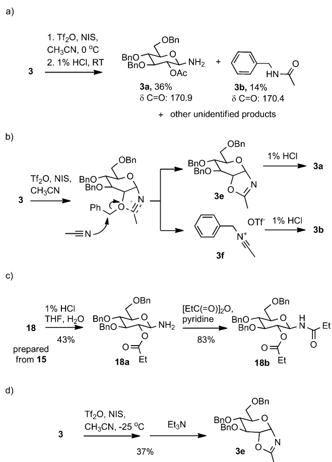
Scheme 2. a) Formation of the 2- O -acetyl glucosylamine 3a and N -benzylacetamide ( 3b ). b) Mechanism for the formation of 3a and 3b . c) Acid hydrolysis of the glucosyl oxazoline 18 . d) Synthesis of the glucosyl oxazoline 3e from fully protected 3 .
