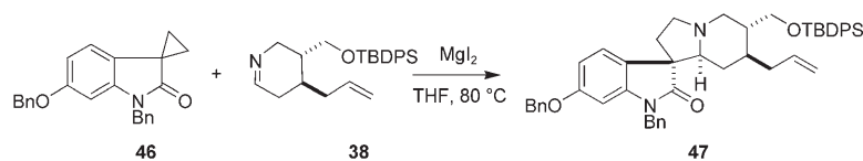
Scheme 8. The critical annulation reaction. a) 1 equiv \text{MgI}_2 , THF, 80^{\circ}\text{C} , 55% (combined yield of the imine forming reaction and the ring-expansion reaction).
