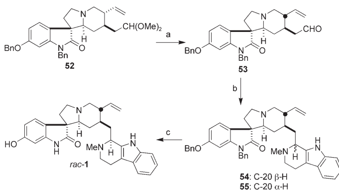
Scheme 10. End steps. a) \text{HCl} (10% in \text{H}_2\text{O} ), acetone, 23^\circ\text{C} , 94% yield; b) \text{AcOH} , toluene, N^m -methyltryptamine, 80^\circ\text{C} , 38% yield for 55 and 26% yield for 54 ; c) \text{Na} in \text{NH}_3 , t\text{BuOH} , THF, -78 to -45^\circ\text{C} , 82% yield.
