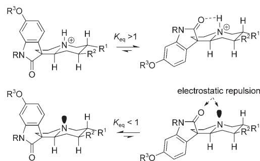
Figure 4. The effect of acidity of the medium on the diastereomer population in the pyrrolidinospirooxindole family of natural products.
