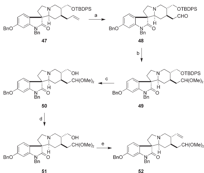
Scheme 9. Synthetic elaboration of 47 . a) i) \text{OsO}_4 , NMO, THF, t\text{BuOH} , \text{H}_2\text{O} , 23^\circ\text{C} ii) \text{NaIO}_4 , THF, t\text{BuOH} , \text{H}_2\text{O} , 23^\circ\text{C} , 86% yield over 2 steps; b) p\text{-TsOH} , \text{MeOH} , \text{CH}(\text{OMe})_3 , 23^\circ\text{C} , 93% yield; c) TBAF, THF, 23^\circ\text{C} , 86% yield; d) IBX, DMSO, 23^\circ\text{C} , 88% yield; e) \text{PPh}_3\text{MeBr} , t\text{BuOK} , THF, 23^\circ\text{C} , 87% yield.
