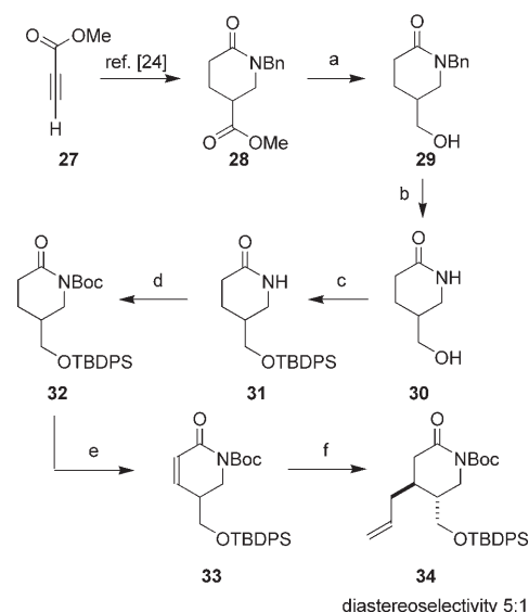
Scheme 5. Synthesis of imide intermediate. a) \text{LiBH}_4 , THF, 23^\circ\text{C} , 88% yield; b) Na, \text{NH}_3 , THF, t BuOH, -40^\circ\text{C} , 10 min, 75% yield; c) imidazole, DMF, TBDPSCl, 23^\circ\text{C} , 91% yield; d) DMAP, \text{NEt}_3 , \text{CH}_2\text{Cl}_2 , \text{Boc}_2\text{O} , 23^\circ\text{C} , 88% yield; e) LHMDS, THF, \text{PhSeCl} , -78^\circ\text{C} , then EtOAc, \text{H}_2\text{O}_2 , 23^\circ\text{C} , 80% yield; f) allylmagnesium chloride, \text{CuBr}\cdot\text{SMe}_2 , THF, -78^\circ\text{C} , 75% yield for both diastereoisomers.
