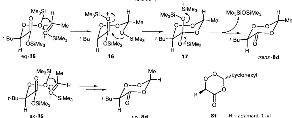
Scheme 4
