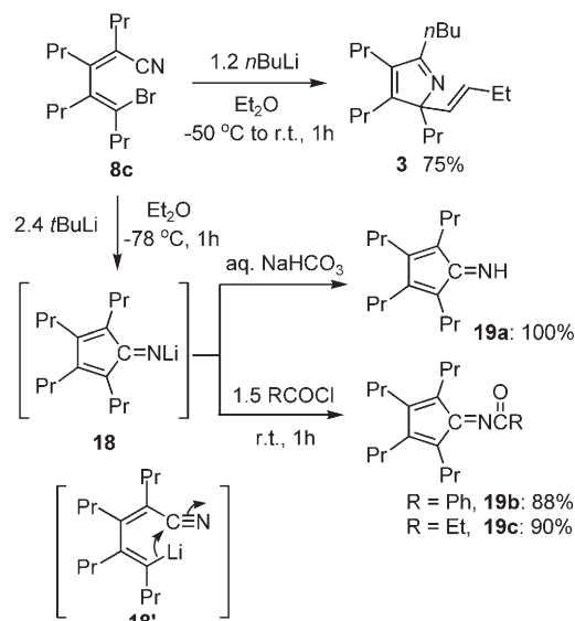
Scheme 7. Reaction of 4-bromodienenenitrile 8c with an organolithium reagent.
