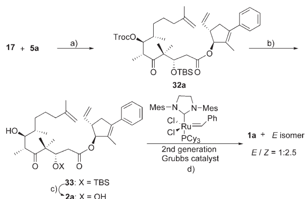
Scheme 10. a) DCC, DMAP, \text{CH}_2\text{Cl}_2 , 0^\circ\text{C} (15 min), RT (16 h), 64%; b) Zn, \text{NH}_4\text{Cl} , anhydrous EtOH, RT, 45 min; c) TAS-F, DMF, 2 d, 62% (2 steps); d) \text{CH}_2\text{Cl}_2 , 50^\circ\text{C} , 16 h, 50% (Z+E). DCC = 1,3-dicyclohexylcarbodiimide, DMAP = 4-dimethylaminopyridine, TAS-F = tris(dimethylamino)sulfur (trimethylsilyl)difluoride.
