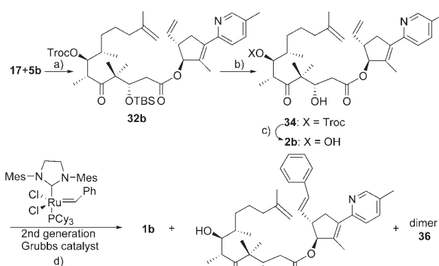
Scheme 11. a) DCC, DMAP, \text{CH}_2\text{Cl}_2 , 0^\circ\text{C} (15 min), RT (16 h), 85%; b) TAS-F, DMF, 2 d; c) Zn, \text{NH}_4\text{Cl} , anhydrous EtOH, RT, 45 min, 62% (2 steps); d) \text{CH}_2\text{Cl}_2 , 50^\circ\text{C} , 16 h, 55%.
