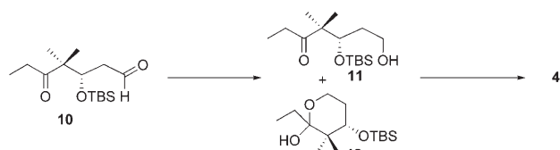
Scheme 3. a) \text{NaBH}_4 , \text{CH}_2\text{Cl}_2 , \text{EtOH} , -78^\circ\text{C} ; b) \text{TBSCl} , imidazole, \text{CH}_2\text{Cl}_2 , 0^\circ\text{C} . \text{TBSCl} = tert -butyldimethylsilyl chloride.
