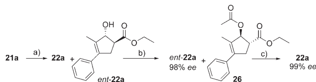
Scheme 7. a) \text{Zn}(\text{BH}_4)_2/\text{ether} , 4^\circ\text{C} , 75 %; b) PS-D lipase, vinyl acetate, 4 Å MS, pentane, RT, 4 d, 48 % ( ent - 22a ), 49 % ( 26 ); c) anhydrous \text{K}_2\text{CO}_3 , anhydrous EtOH, RT, 12 h, 92 %. MS = molecular sieves.
