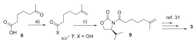
Scheme 2. a) \text{MeP}^+(\text{Ph})_3\text{Br}^- , n\text{BuLi} , DMSO/THF, RT, 48 h, 78 %; b) (\text{COCl})_2 , benzene; c) ( S )-4-isopropyl-2-oxazolidonone, n\text{BuLi} , THF, -78^\circ\text{C} .
